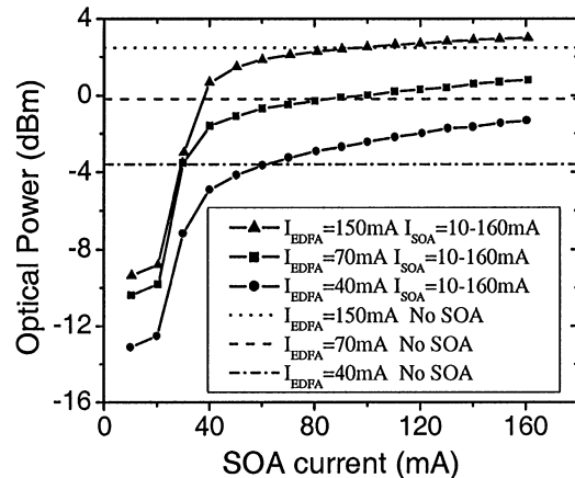
Fig. 6. Optical power of the laser output light under several EDFA and SOA currents.
