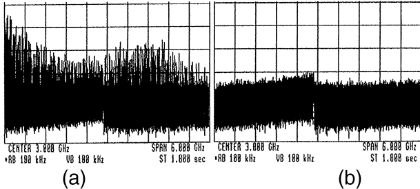
Fig. 3. rf spectrum of the light output from the laser in Fig. 1: (a) without and (b) with a SOA in a 0–6-GHz span (vertical scale, 10 dB/division).
