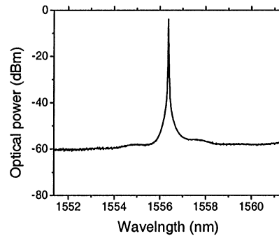
Fig. 5. Output optical spectrum of the laser in Fig. 1 with a SOA.
