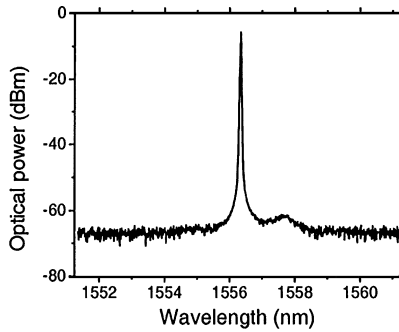
Fig. 2. Output optical spectrum from the laser in Fig. 1 without a SOA.
