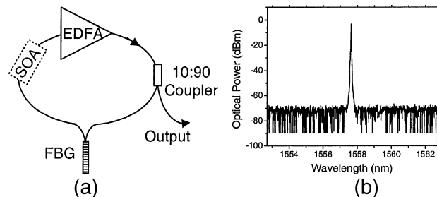
Fig. 7. (a) FBG-based fiber ring laser and (b) output optical spectrum without a SOA.
