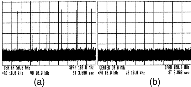
Fig. 4. rf spectrum of the light output from the laser in Fig. 1: (a) without and (b) with a SOA in a 0–100-MHz space (vertical scale, 10 dB/division).
