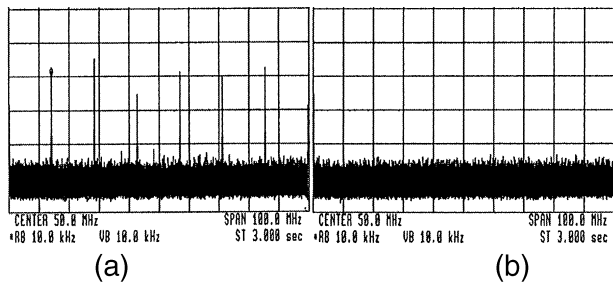
Fig. 8. rf spectra from a FBG-based erbium-doped fiber ring laser: (a) without and (b) with a SOA in a 0–100-MHz span (vertical scale, 10 dB/division).
