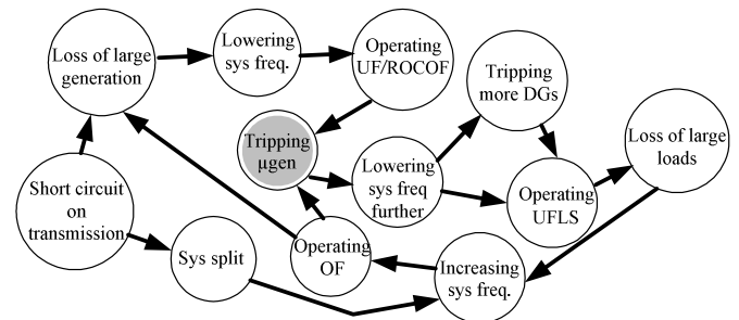
Fig. 1. The sequences of the events accompanying a frequency disturbance
