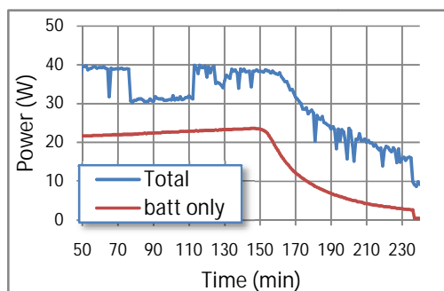
Figure 1 - Power Profile of a Representative BIEN-RPG Compatible Portable ICT Device
