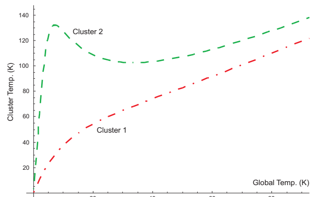
FIG. 3: A plot of the temperatures of two interacting sub-systems consisting of several electrons with Coulomb exchange energy.
