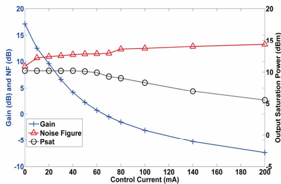
Figure 2. Modeled steady state AGC-SOA performance.
