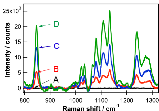
Fig. 3 Ensemble SERRS spectra of samples A, B, C, and D using an excitation wavelength of 785 nm and accumulation time of 10 s.
