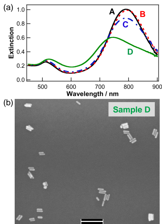
Fig. 2 UV-vis spectra of four PSS-wrapped samples A, B, C and D. Differences between each sample are described in the main text and ESI † . (b) Representative SEM image of sample D (scale bar = 200nm).
