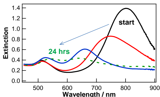
Fig. 1 Spectra monitoring the controlled side-by-side assembly of gold nanorods following the addition of citrate anions to a nanorod solution. The resulting plasmon resonance shifts were measured over 24 hrs.
