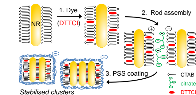
60 Scheme 1 Schematic outlining the preparation and stabilisation of self-assembled gold nanorod/dye clusters.
