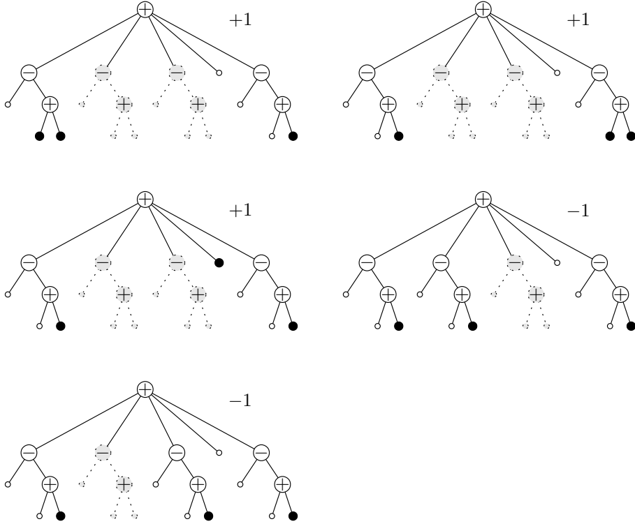
FIGURE 2. The normal embeddings of \sigma in \pi (see Figure 1), together with their signs. The leaves covered by the embedding are represented by black disks, the leaves that are maximal omitted are represented by empty circles. Dotted lines represent subtrees rooted at a maximal omitted internal node. Note that the leaves of such subtrees do not contribute to the sign of the embedding.
