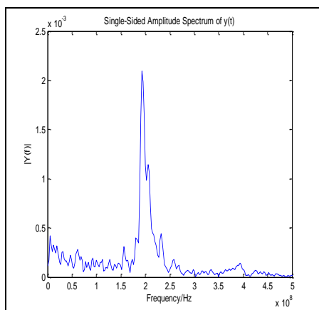
Fig. 7b spectrum from IEC measurements for PVC at 3.75 kV
