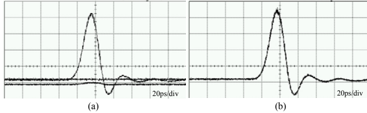
Fig. 6. Amplified switched MZIS output as seen by the bandwidth limited oscilloscope. (a) overlaid picture when both cw and clock are ON, clock ON and cw ON only; (b) - switched output after MZIS was temperature tuned to the next dark fringe.
