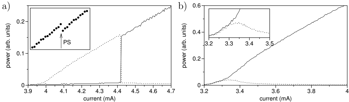
Figure 3: Polarization resolved output power in dependence of the injection current. a) PS at a substrate temperature of 10^{\circ}\text{C} . The inset displays a magnification of the total output power (dotted line) in the vicinity of the PS, measured without polarization sensitive optics. b) TFE at a substrate temperature of 61^{\circ}\text{C} . The inset shows a magnification of the current interval around threshold. (From [42, 44])
