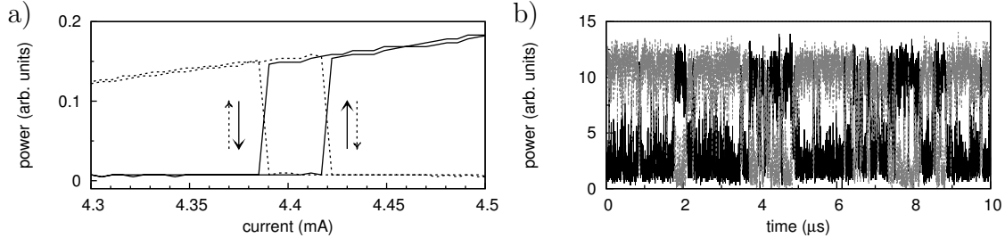
Figure 5: a) Polarization resolved LI-curve including the measurement for increasing and decreasing current (substrate temperature 10^\circ\text{C} ). The arrows indicate the direction of the polarization switching. The scanning time for the complete measurement is 160 seconds. b) Time series with a cw bias within the bistable range (substrate temperature 40^\circ\text{C} , grey line LF-mode, black line HF-mode).
