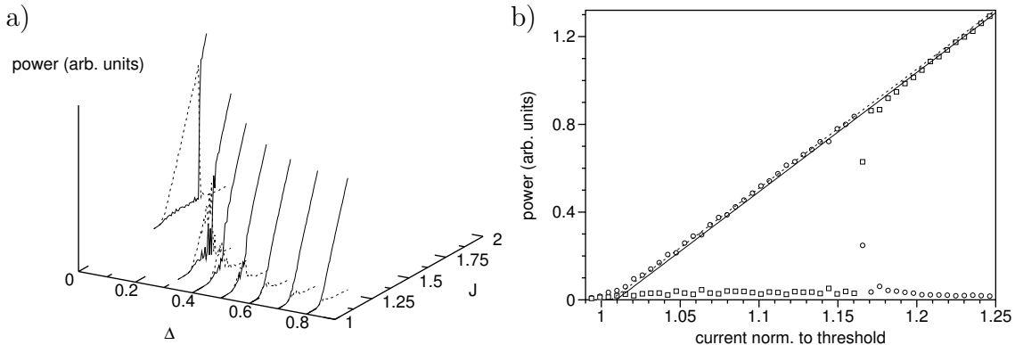
Figure 9: a) Polarization resolved output power in dependence of the detuning \Delta and injection current J normalized to its transparency value. The parameters defining the susceptibility function [67] are b = 10^4 , \gamma_{\perp} = 10^4 \text{ ns}^{-1} , and \sigma = 0.2 , other parameters \gamma_p = 18 \text{ ns}^{-1} , \gamma_a = 0 , \kappa = 300 \text{ ns}^{-1} , a = 2.3 \cdot 10^4 \text{ ns}^{-1} , \Gamma = 0.045 , A = 0.5 \text{ ns}^{-1} , B = 1.0 \text{ ns}^{-1} , \beta_{sp} = 10^{-6} \text{ ns}^{-1} , \gamma_j = 20 \text{ ns}^{-1} . b) Polarization resolved LI-curve obtained from simulations for \Delta = 0 . Circles (squares) denote the power in the mode with higher (lower) optical frequency. The dashed (solid) lines are linear fits applied to the data before (after) the PS. The integration time per point is 100 ns. (From [42, 44])
