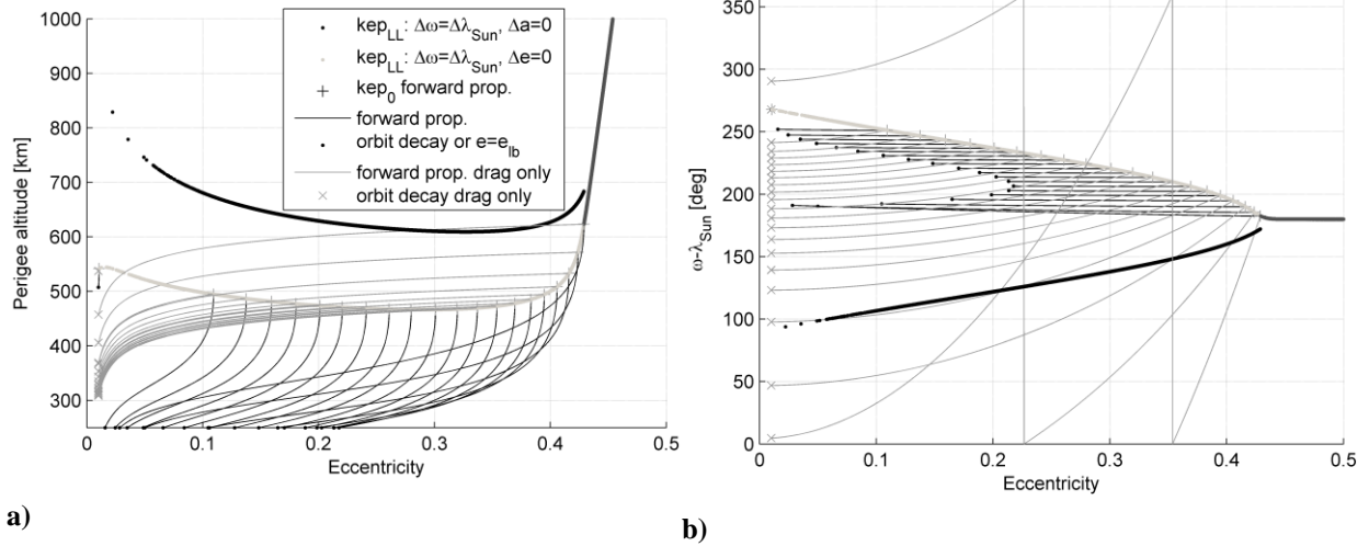
Fig. 13 Long-term orbit evolution for SpaceChip 3 from initial conditions with \Delta e=0 and \Delta\omega=\Delta\lambda_{Sun} . The black lines represent the SRP and drag case, the gray lines the drag-only case.
