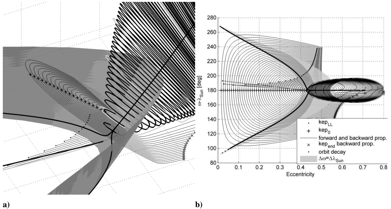
Fig. 24 Long-term orbit evolution for SpaceChip 3 for condition with librational and progressively decaying motion . a) Zoom on the bifurcation region, and b) 2D view in eccentricity – \omega - \lambda_{\text{Sun}} .
