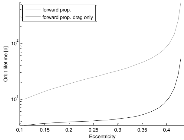
Fig. 14 SpaceChip 3 orbit lifetime for evolution from initial conditions with \Delta e=0 and \Delta\omega=\Delta\lambda_{Sun} . The vertical axis is in logarithmic scale. The black line represents the SRP and drag case, the gray line the drag-only case.
