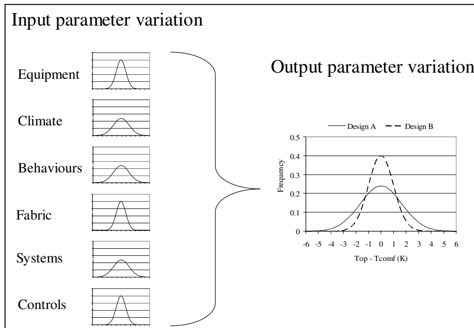
Figure 9 The variation in input parameters combined in dynamic simulation using Monte-Carlo method to give a resulting variation in output parameters for Design A and Design B (see also Figure 10).
