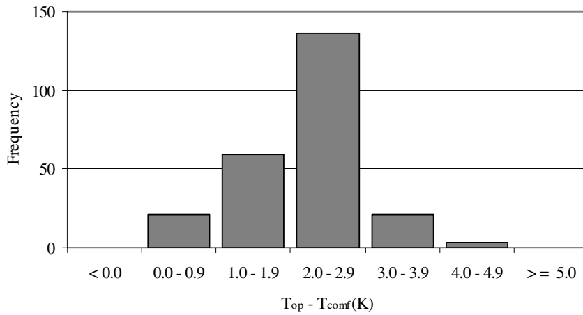
Figure 8 The predicted distribution of the deviation from optimal thermal comfort temperature ( T_{op} - T_{comf} ) for the same summer day as in Figure 10 due to the variation in occupant behaviour as embedded in the Humphreys algorithm.
