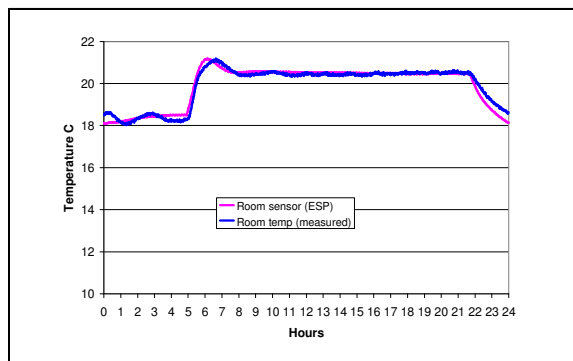
Figure 9 Time proportional PI controller room temperature comparison.
