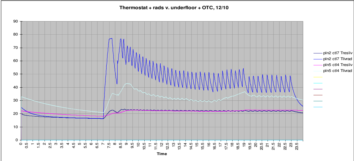
Figure 10 Comparison of thermostat and radiator system with underfloor heating and weather compensation.
