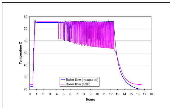
Figure 6 On/off thermostat boiler water temperature comparison.
