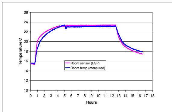
Figure 5 On/off Thermostat room temperature comparison (test room 1).
