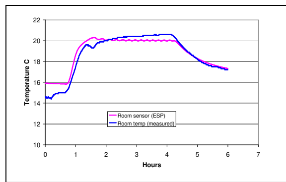
Figure 7 PI controller room temperature comparison
