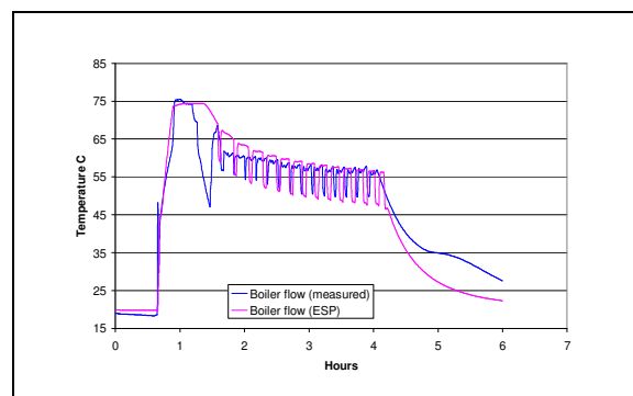
Figure 8 PI controller boiler temperature.
