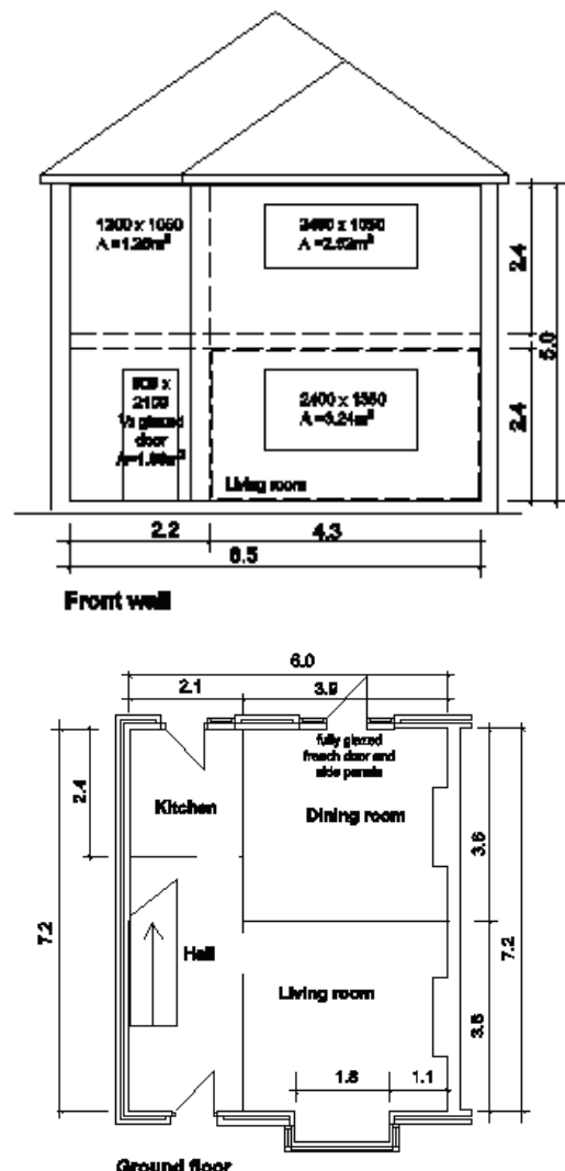
Figure 2 Elevation and ground floor plan for semi-detached house.
