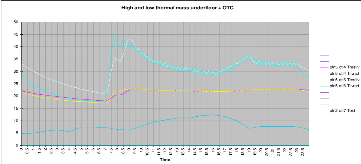
Figure 11 Comparison of high and low thermal capacity underfloor heating with weather compensation.
