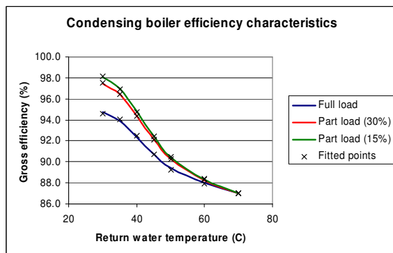
Figure 3 Efficiency characteristics for a condensing gas boiler.
