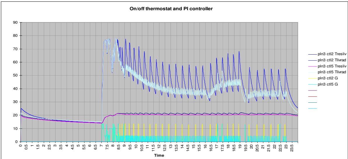
Figure 12 Comparison of on/off thermostat and PI room controller.
