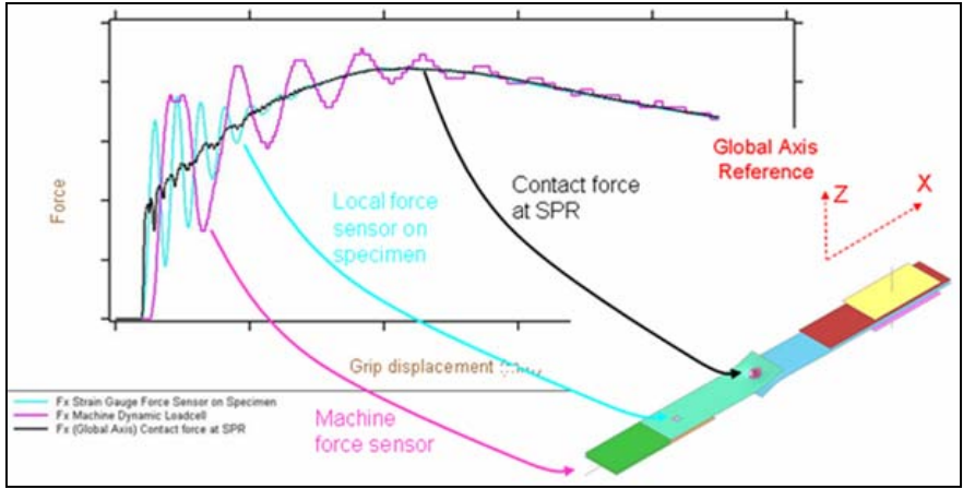
Figure 11a: Comparing force measurement locations from lap shear model in global axis reference
