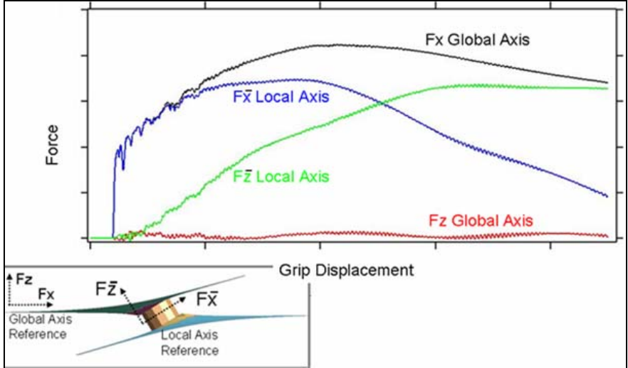
Figure 11b: Comparing measurements in global and local axis reference systems at connection
