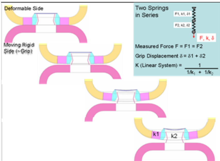
Figure 7a: U-tension model may be represented by series spring with 2dof
