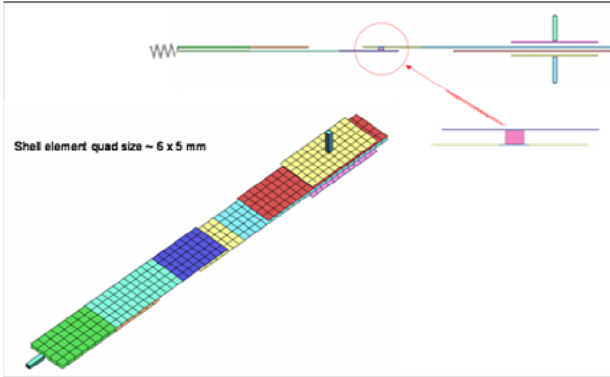
Figure 13a: Lap shear engineering scale model, connection modelled with discrete beam
