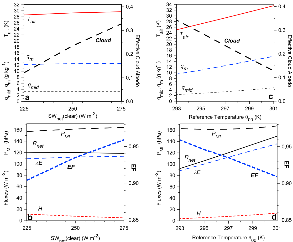
Figure 1. Sensitivity of (a) T_{\text{air}} , q_{\text{m}} , q_{\text{mid}} , and effective cloud albedo, (b) surface fluxes, EF and ML depth to SW_{\text{net}}(\text{clear}) . (c and d) Same as Figures 1a and 1b for sensitivity to reference temperature, \theta_{00} .
