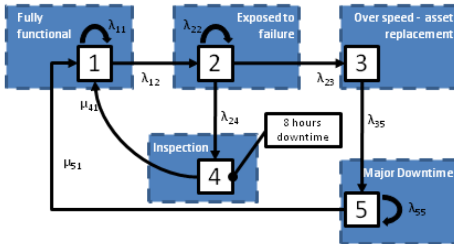
Fig. 4. Over Speed State Space Diagram
