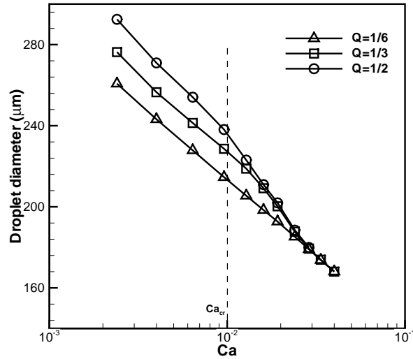
Figure 11: The effect of capillary number and flow rate ratio on droplet diameter at a fixed viscosity ratio, \lambda=1/4 . Note that, for Q=1/2 and Ca > 0.024 , the measured droplet diameters are not plotted in this figure due to irregular droplets are generated.
