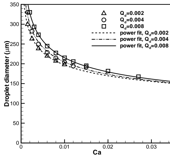
Figure 8: The influence of capillary number on the droplet diameter at the dispersed phase flow rate Q_d of 2 \times 10^{-3} , 4 \times 10^{-3} and 8 \times 10^{-3} respectively. The lines represent the power fittings of the simulation results.
