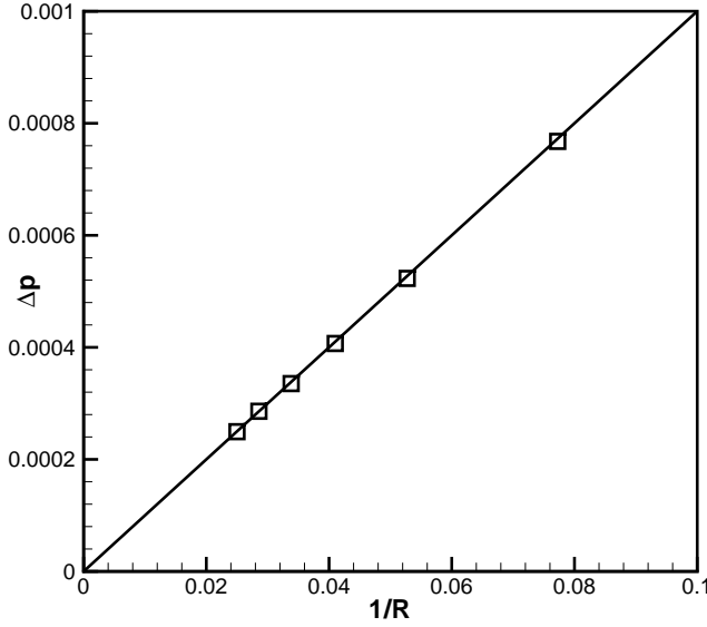
Figure 1: Comparison of the LBM results ( \square ) with the Laplace's law (the solid line) for pressure jump across a stationary droplet interface.
