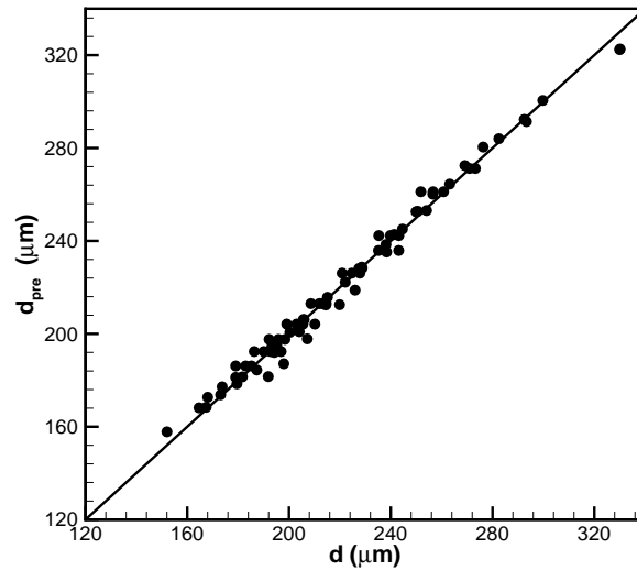
Figure 15: Comparison of droplet diameter between the fitting results d_{pre} from Eq. (4.2) and the simulation results d .
