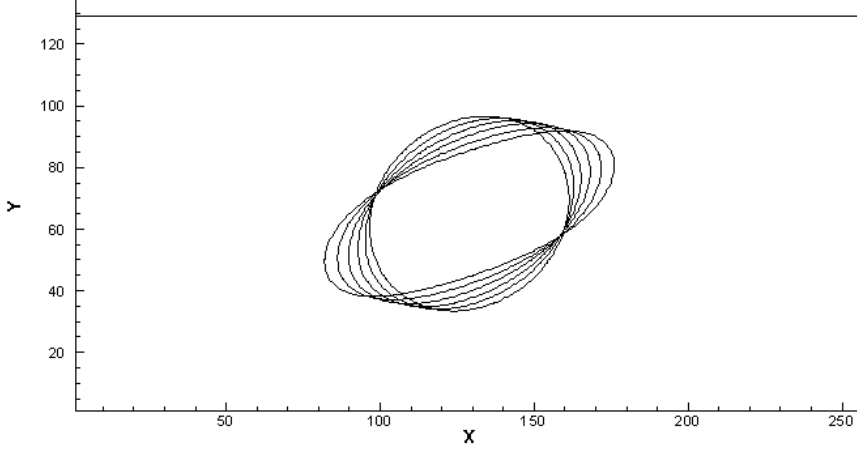
Figure 5: Stable droplet shape depicted as contour lines of \phi = 0 , for various capillary numbers: Ca = \{0.05, 0.1, 0.15, 0.2, 0.25, 0.3\} .
