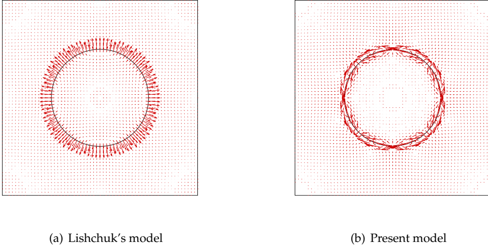
Figure 3: Comparison of the spurious velocities of a droplet in stationary fluid with \sigma=0.01 and R=30\delta_x for (a) the model proposed by Lishchuk et al. [41] with the magnification rate of 1:1.5\times 10^5 and (b) the present model with the magnification rate of 1:1.5\times 10^7 .
