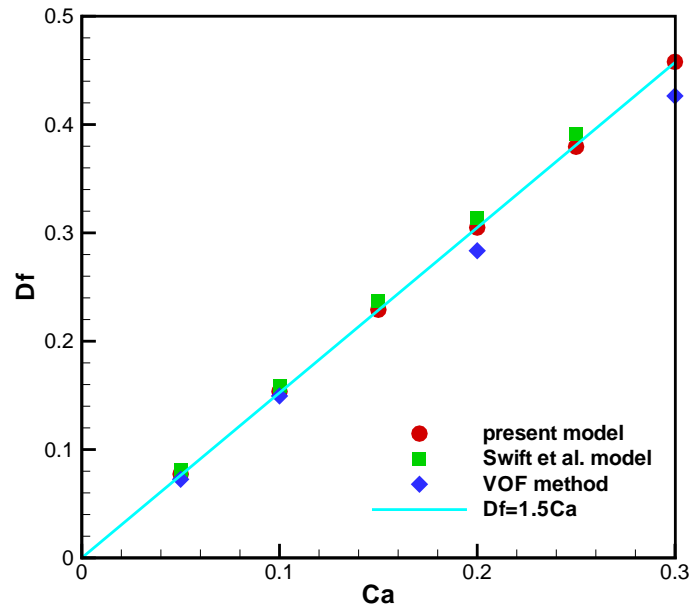
Figure 4: Taylor deformation parameter Df as a function of the capillary number.
