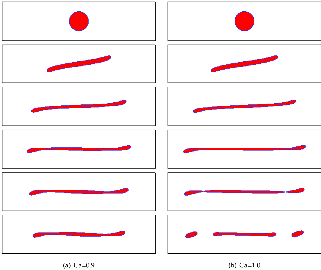
Figure 6: Snapshots of the droplet evolution under simple shear flow at \lambda=1 , Re=1.0 for (a) Ca=0.9 and (b) Ca=1.0 , taken at times T=\{0,6,12,24,27,30\} .
