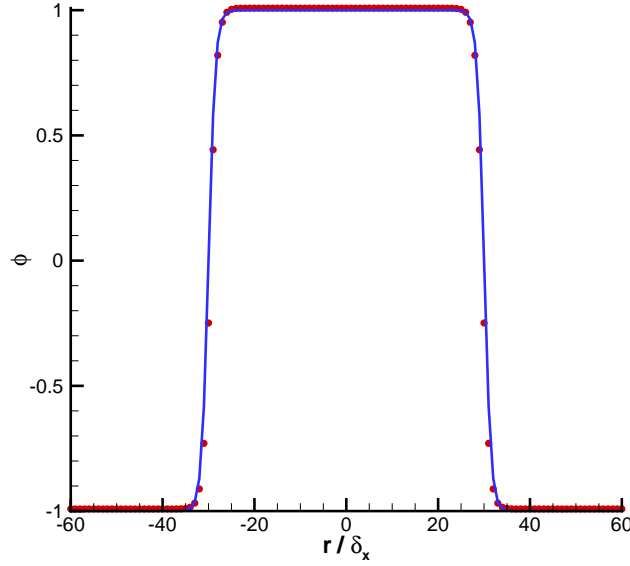
Figure 2: The profile of order parameter along the cross section of a droplet with R=30\delta_x . The discrete symbols represent the simulation results of the present LB model and the solid line is the theoretical profile given by Eq. (3.2).
