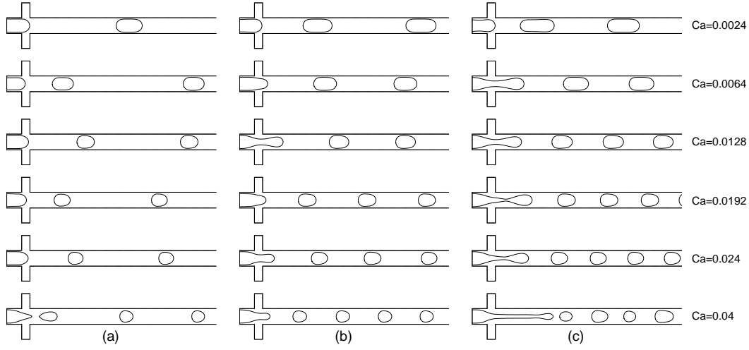
Figure 10: The flow patterns for various capillary numbers and the flow rate ratios at a fixed viscosity ratio \lambda = 1/4 : (a) Q = 1/6 ; (b) Q = 1/3 ; and (c) Q = 1/2 . Each row uses the same capillary number, which is labelled on the right side.
