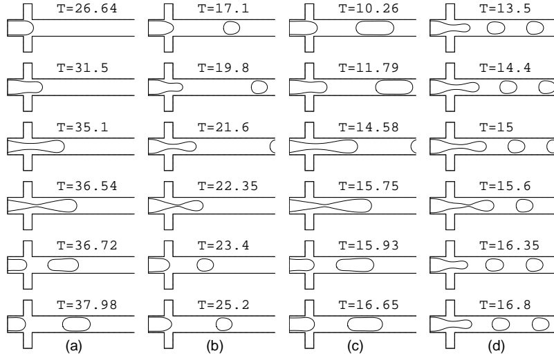
Figure 12: A series of instantaneous states of droplet formation for (a) Q=1/6 , Ca=0.0024 ; (b) Q=1/6 , Ca=0.024 ; (c) Q=1/2 , Ca=0.0024 and (d) Q=1/2 , Ca=0.024 . The viscosity ratio \lambda=1/4 , and the dimensionless time is defined as T = \frac{u_c}{w_c} t .
