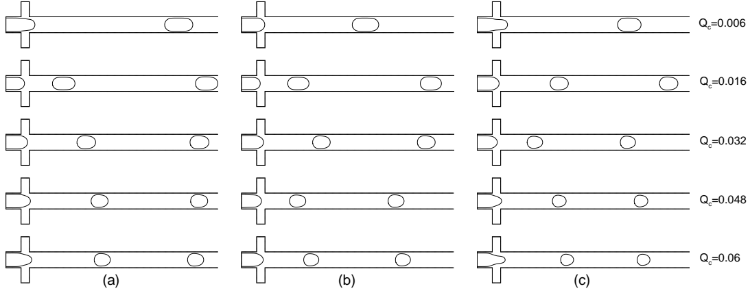
Figure 14: The flow patterns for various \eta_c and Q_c at a fixed flow rate ratio Q=1/6 : (a) \eta_c=0.06 ; (b) \eta_c=0.08 ; and (c) \eta_c=0.16 . Each row uses the same Q_c , which is labeled on the right side.
