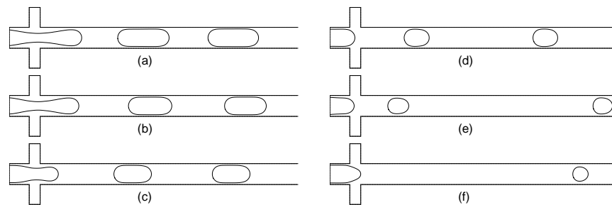
Figure 9: The droplet generation at the dispersed phase flow rate Q_d = 8 \times 10^{-3} for various capillary numbers: (a) 0.002; (b) 0.003; (c) 0.004; (d) 0.01; (e) 0.02; and (f) 0.035.
