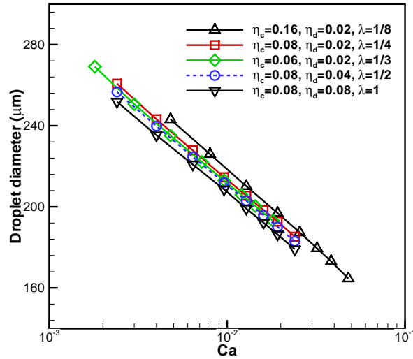
Figure 13: The effect of capillary number and viscosity ratio on droplet diameter at a fixed flow rate ratio, i.e. Q=1/6 .
