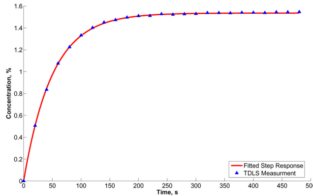
Figure 2: Time evolution of the methane concentration from one of the bleed lines after the selection valve has been changed.
