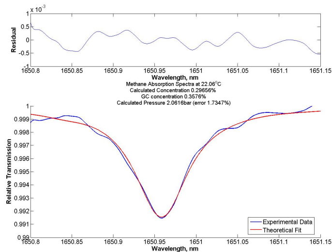
Figure 4: TDLS concentration and pressure measurement for the reformer outlet, and a comparison with the GC
