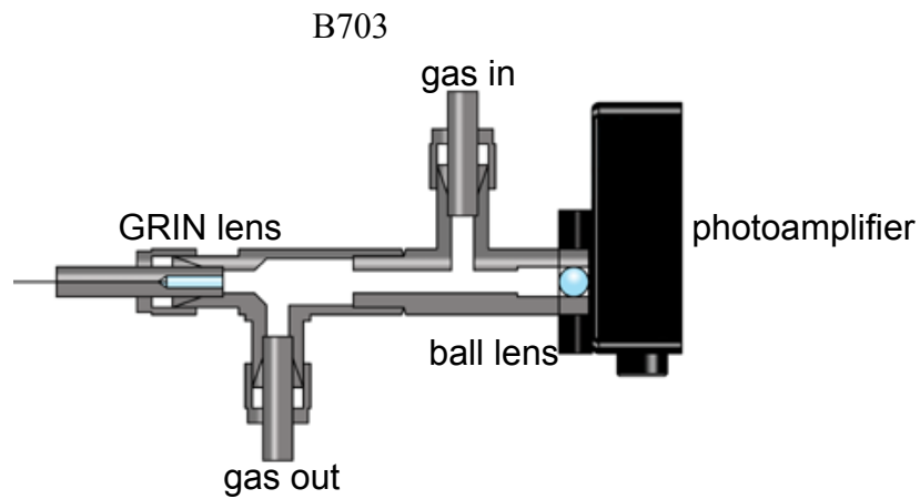
Figure 1: In-line gas analyser. Light enters through the GRIN lens, and is focused onto the photodiode using a sapphire ball lens. Gas passes through the cell via the inlet and outlet Swagelok piping.
