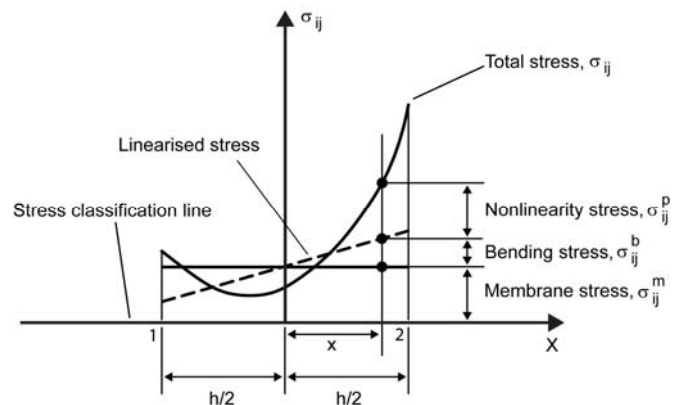
Figure 1 - Typical stress distribution along a classification line
