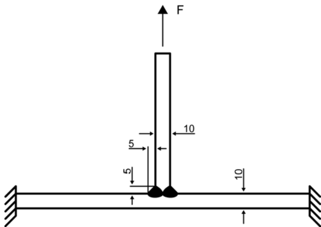
Figure 4 - T shaped welded plates under bending
