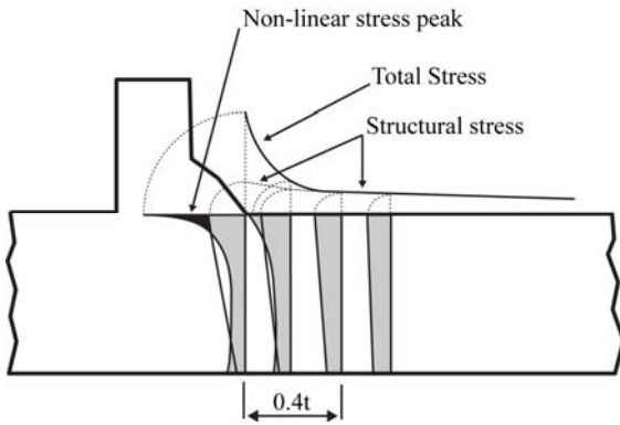
Figure 2 - Surface distribution across the plate thickness and along the surface in the vicinity of the weld, adapted from [3]
