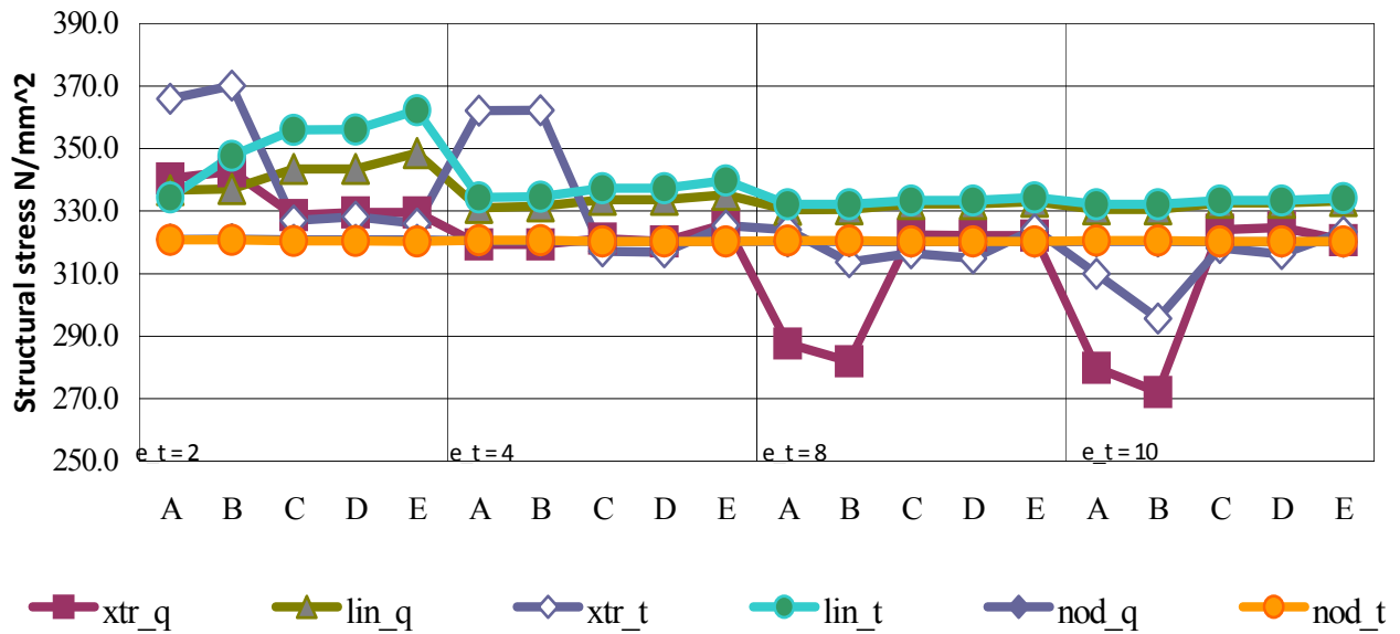
Figure A.1 – T-shaped welded plates - Structural stresses
