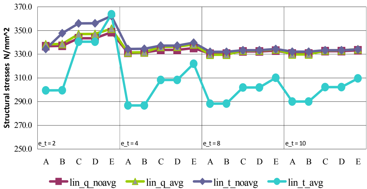
Figure A.2 - T-shaped welded plates - Structural stresses (averaged and unaveraged)- linearization through thickness
