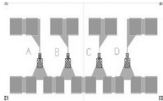
Fig. 5. Sketch of the 4-device layout on a 5 mm \times 10 mm chip. Hatched rectangles represent the Au-film resistors.
