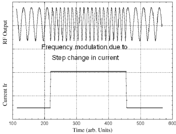
Fig. 2. Example of time-domain simulation of an R-SQUID, obtained by JSIM. The response of the heterodyne frequency to a step change in the current I_r is illustrated.
