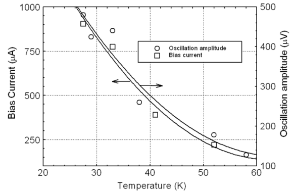
Fig. 8. The junction optimum bias currents (open squares, left axis) and the heterodyne oscillation amplitudes (open circles, right axis) have similar temperature dependences. The solid lines are best quadratic fits to the two data sets.
