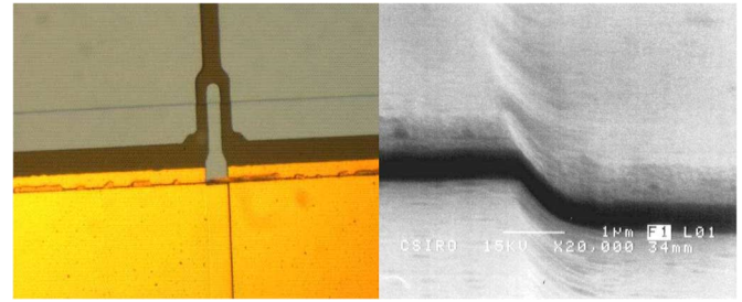
Fig. 4. A photograph of a fabricated device junction area (left) and an SEM micrograph of the YBCO step-edge junction (right). The step, produced on the MgO substrate by Ar-ion beam etching, is \sim 400 nm in height. The magnification is \times 20,000 .
