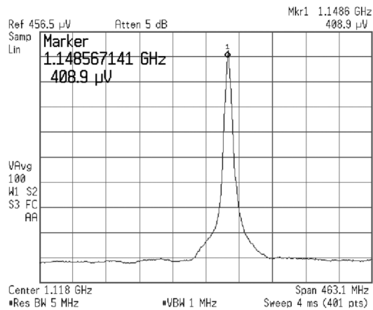
Fig. 6. Spectrum analyser trace obtained by suitable adjustment of the bias current I_j . A low-noise broadband rf pre-amplifier (gain 20 dB) was used.
