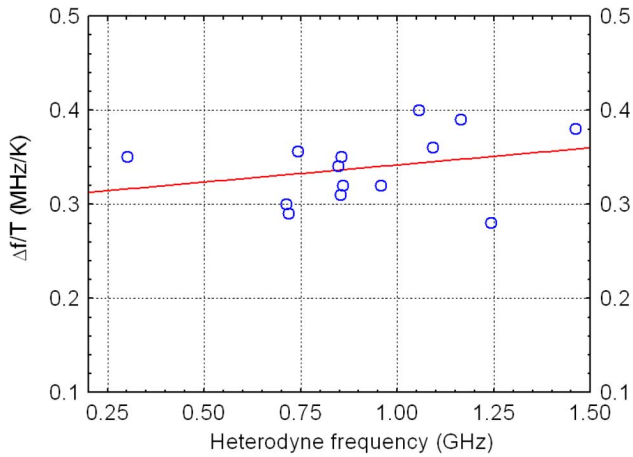
Fig. 10. The linewidth/temperature ratio showed a weak dependence on the heterodyne frequency.
