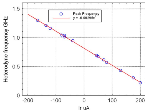
Fig. 7. Dependence of heterodyne frequency on current I_r applied to the resistor R_s at T = 27 K. Negative slope is due to arbitrary choice of polarity of current connections.
