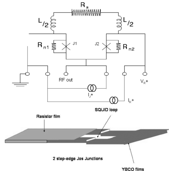
Fig. 1. (Upper), schematic circuit of R-SQUID device; components are explained in the Text; (lower:), sketch of thin-film geometry used to produce the R-SQUID.
