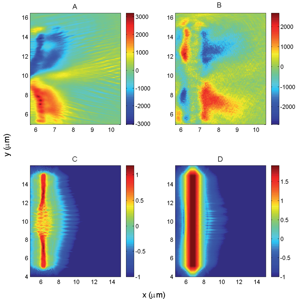
Figure 5. Plots of magnetic flux density, B_z (T), in simulation of 80 nm ‘CH’ target (a) and 1 \mu\text{m} (b) at 200 fs. Plots of proton density ( \log_{10}(n_p/n_{crit}) ) in simulation of 80 nm ‘CH’ target (c) and 1 \mu\text{m} (d) at 200 fs. Foil is initially positioned at x = 6.05 \mu\text{m} . Note that a region where B_z > 1000 T extends 1–2 \mu\text{m} away from the rear surface.
