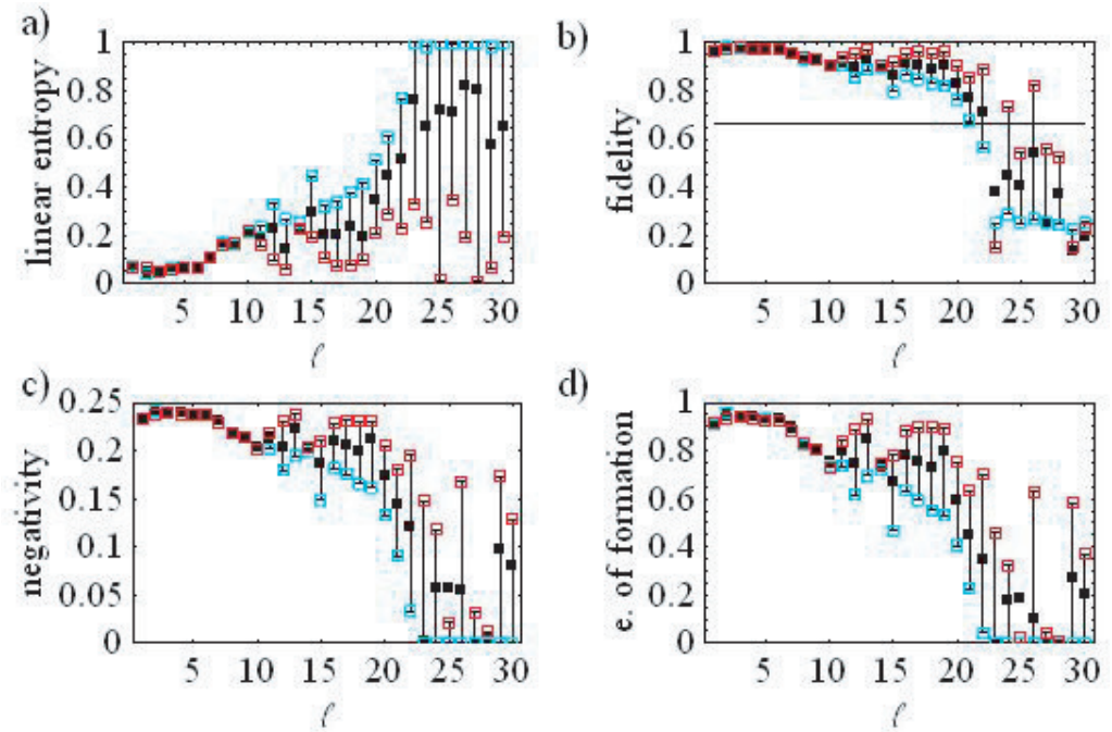
Figure 6. Various measures of state purity and entanglement for OAM subspaces between |\ell| = 1 and 30, and the maximum (red) and minimum (cyan) level consistent with the measurements. Horizontal lines indicate the border between entangled and mixed states. Strong entanglement persists up to an OAM of about 20.
