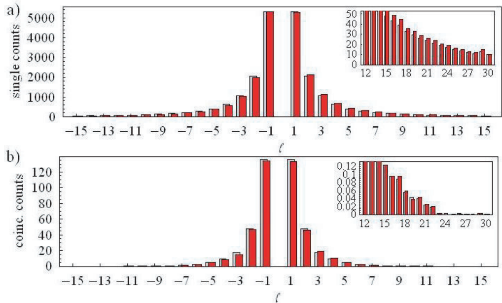
Figure 1. The generation of OAM modes tails off with increasing |\ell| . This can be seen both in the singles count rates (a) and the coincidence count rates (b). The red bars show the count rates proportional to |a_{\ell,-\ell}|^2 , and the grey bars (|a_{-\ell,-\ell}|^2 + |a_{\ell,-\ell}|^2 + |a_{-\ell,\ell}|^2 + |a_{\ell,\ell}|^2)/2 for the coincidence counts and similarly for the single count rates. From the insets it is clear that the coincidence count rates become comparable to the noise level for |\ell| > 22 .
