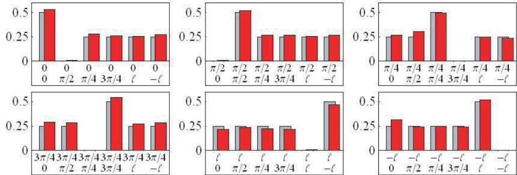
Figure 4. Characterization of the two-photon state by 36 correlation measurements of simultaneously detecting each photon in one of the six measurement states (red), and ideal values expected for a maximally entangled state and perfect measurements (grey). Shown are the results for the subspace |\ell| = 3 .
