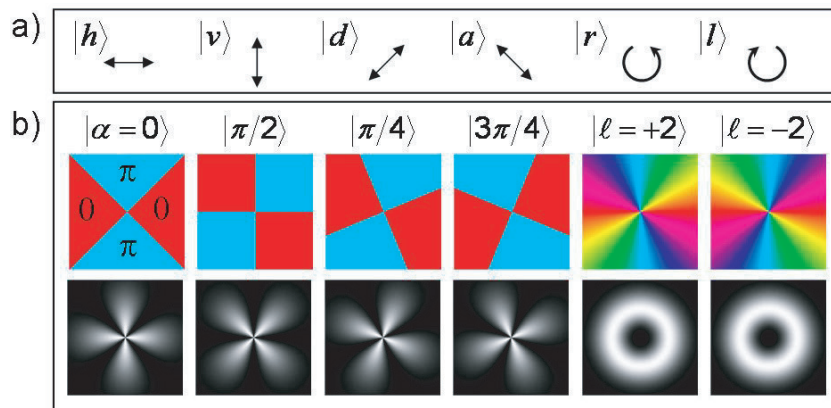
Figure 2. Different basis states describing the polarization of light (a) and the equivalent states for the OAM of light (b), here shown for the |\ell| = 2 subspace. Shown are the phase profiles (top) and intensity profiles (bottom).
