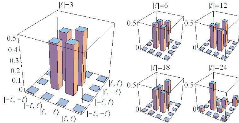
Figure 5. Graphical representation of the real part of the density matrix for various |\ell| subspaces. For subspaces of |\ell| \leq 22 the four central entries of the density matrix dominate, indicating quantum entanglement. For larger \ell the coincidence counts become comparable to the noise background and quantum correlations deteriorate.
