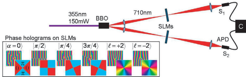
Figure 3. Experimental set-up. SLMs imaged onto avalanche photo detectors (APDs) allow us to perform projection measurements onto the six states |0\rangle , |\pi/2\rangle , |\pi/4\rangle , |3\pi/4\rangle , |+2\rangle and |-2\rangle . We record single ( S_1 and S_2 ) as well as coincidence counts ( C ).
