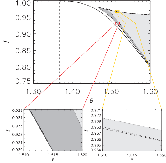
Fig. 9. Projection in the (I, \theta) plane of the saddle-nodes for low-order localized states found in the Kerr-cavity. [Reprinted figure with permission from Gomila et al. (2007). Copyright 2007 of Elsevier Science.]
