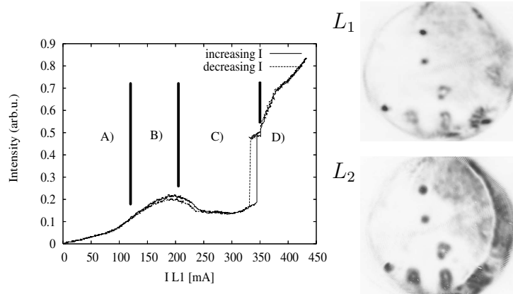
Fig. 23. Left panel: Local intensity output emitted by the system when the current I_{L1} is scanned in the gain device for all the other parameters constant. A) below threshold, B) lasing by feedback, C) absorption by L_2 , bistable behavior, D) pattern formation. Right panel: Examples of near field intensity distributions in both devices in region C showing LCS (upper one gain device; lower one absorber). L_2 is slightly shifted on the left. Dark areas correspond to high intensities. (Courtesy of P. Genevet, adapted from Genevet et al. (2008))
