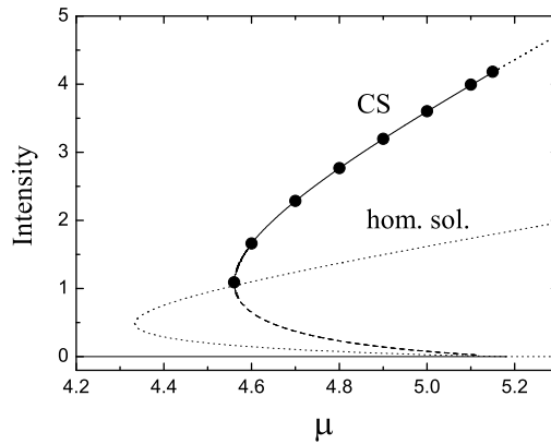
Fig. 22. Local intensity versus pumping parameter in gain section for a LSA. The characteristics are obtained for a semiconductor nonlinearity but serve to illustrate a more general phenomenology. Light dotted lines: homogenous state. Solid line: stable SDS branch. Dashed line: Unstable SDS branch. ( Courtesy of F. Prati, adapted from Prati et al. (2007) ).
