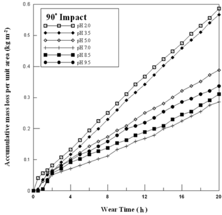
Fig. 13 - Accumulated mass loss curves at 90° ( \text{kg m}^{-2} )
