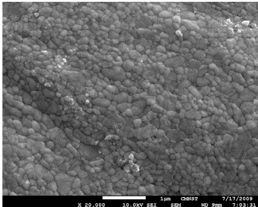
Fig. 11 - SEM observation of Y-TZP specimen after impact by solid particles at 45° after 20h (Section 3)
