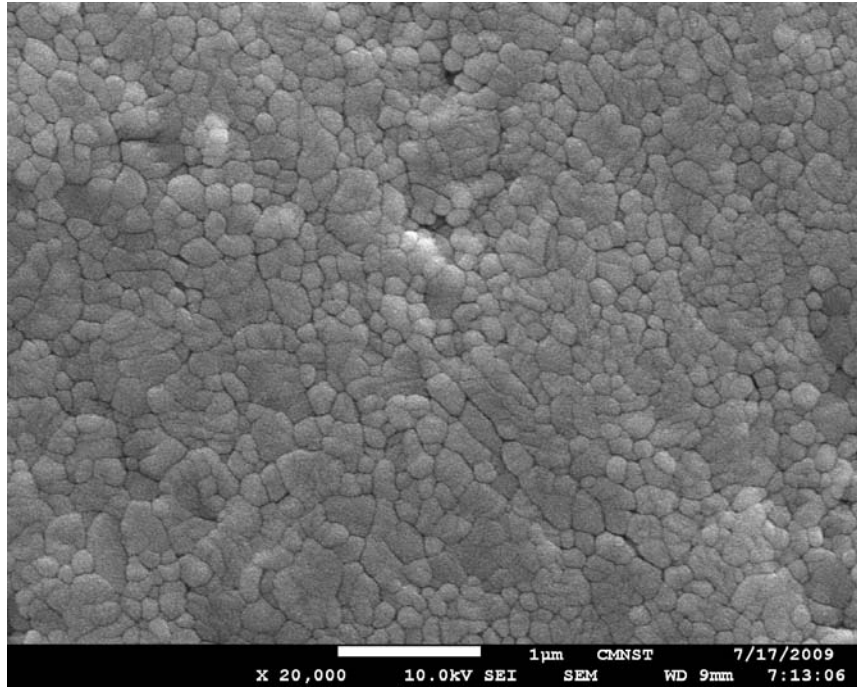
Fig. 12 - SEM observation of Y-TZP specimen after impact by solid particles at 60° after 20h (Section 3)
