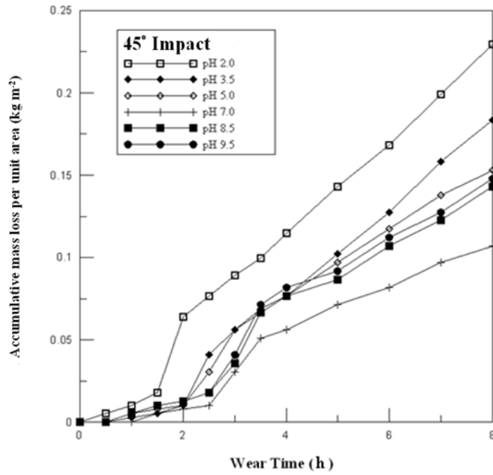
Fig. 16 - Accumulated mass loss curve at 45° (kg m -2 )
