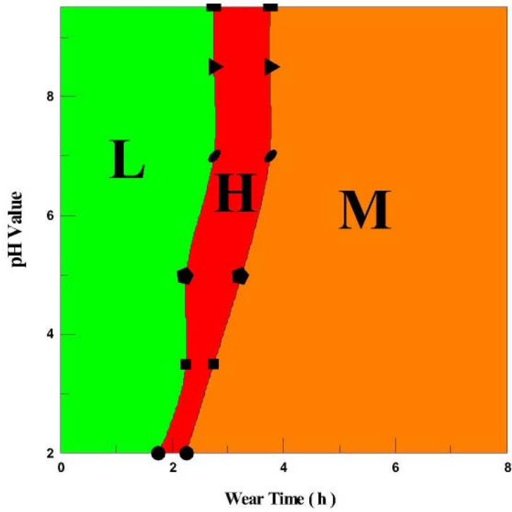
Fig. 21 - Wear rate map at 30° (Green: Low, Orange: Medium, Red: High)
