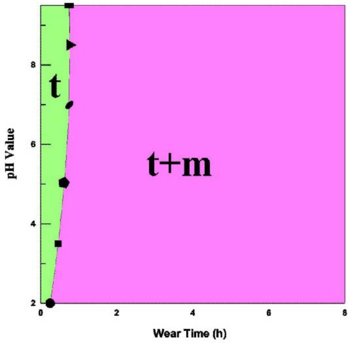
Fig. 24 - Wear phase transformation map at 90° (Light Green: Tetragonal, Pink:
