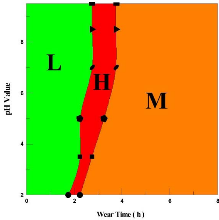
Fig. 22 - Wear rate map at 45°(Green: Low, Orange: Medium, Red: High)
