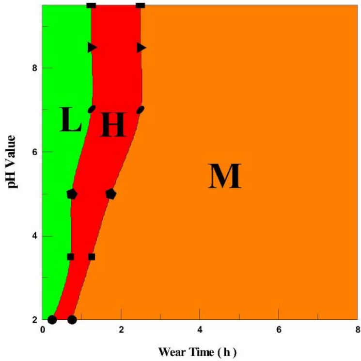
Fig. 19 - Wear rate map at 90° (Green: Low, Orange: Medium, Red: High)
