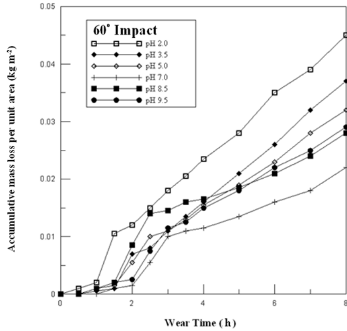
Fig. 17 - Accumulated mass loss curve at 60° (kg m -2 )
