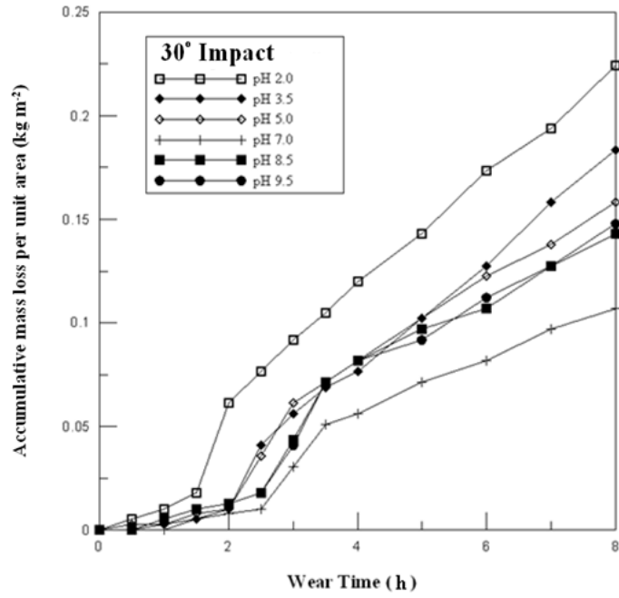
Fig. 15 - Accumulated mass loss curve at 30°(kg m -2 )
