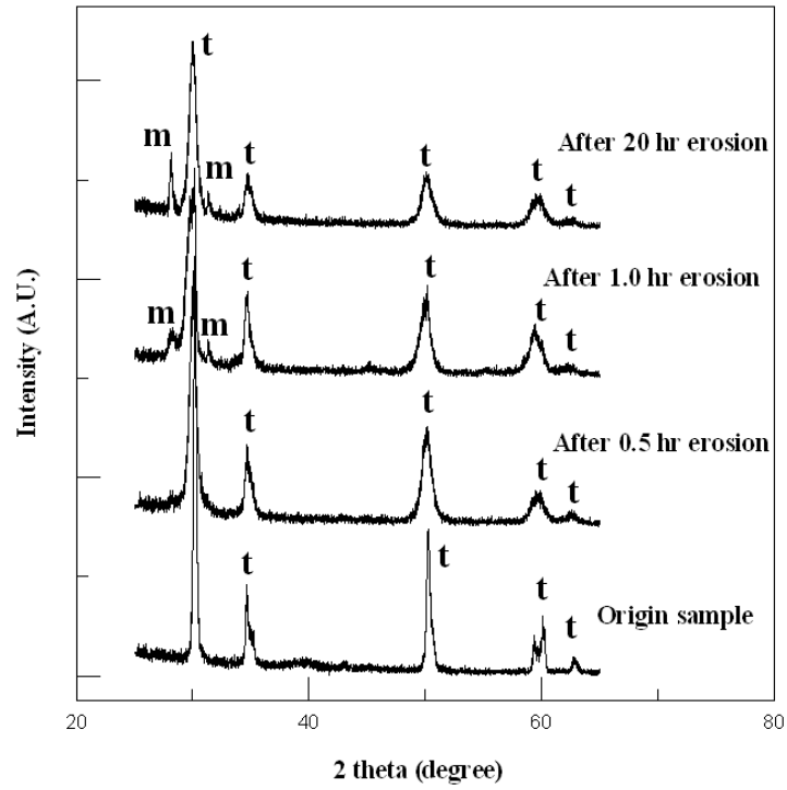
Fig. 4 - XRD analysis of the specimens eroded at pH 9.5 at 90° (Section 3)
