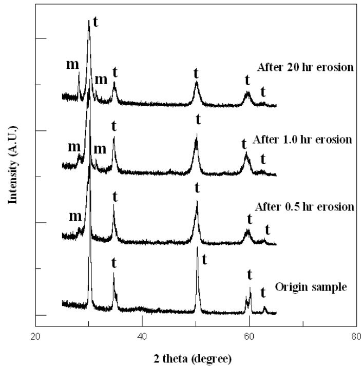
Fig. 5 - XRD analysis of the specimens at pH 9.2 at 90° (Section 3)
