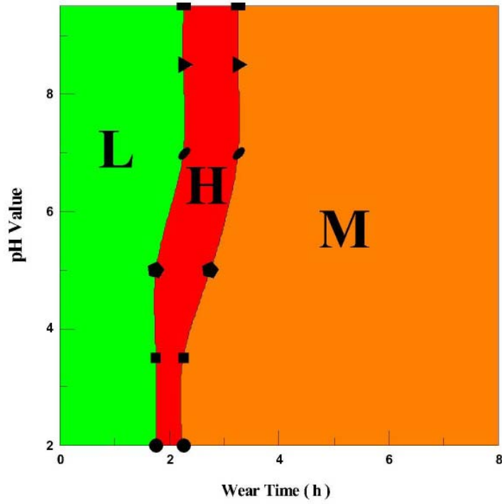
Fig. 23 - Wear rate map at 60°(Green: Low, Orange: Medium, Red: High)
