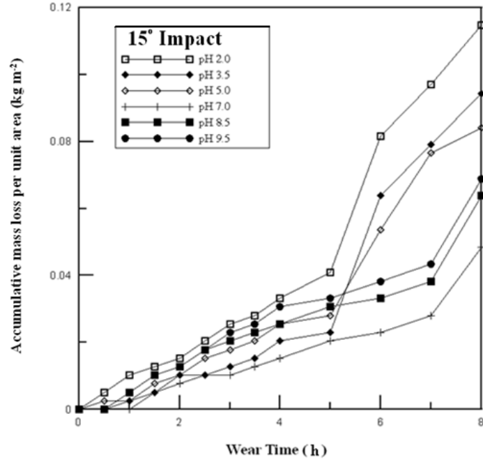
Fig. 14 - Accumulated mass loss curve at 15° ( \text{kg m}^{-2} )
