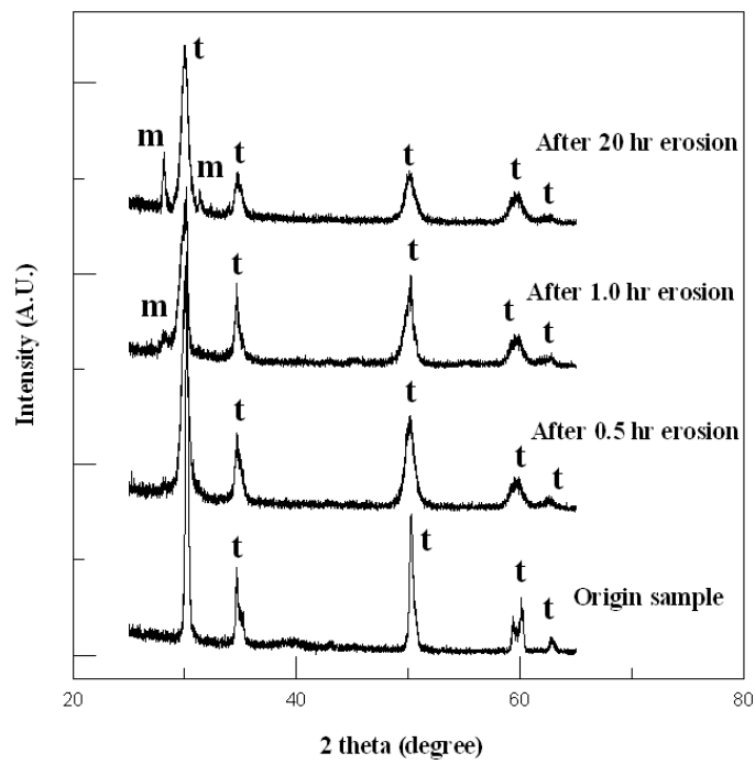
Fig. 3 - XRD analysis of the specimens eroded at pH 7.0 at 90° (Section 3)
