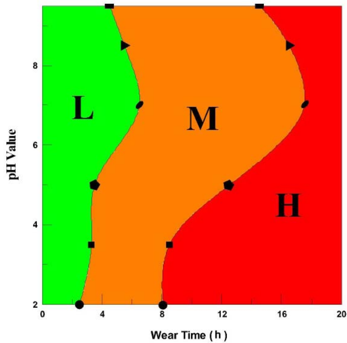
Fig. 18 - Wear map at 90° (Green: Low, Orange: Medium, Red: High)
