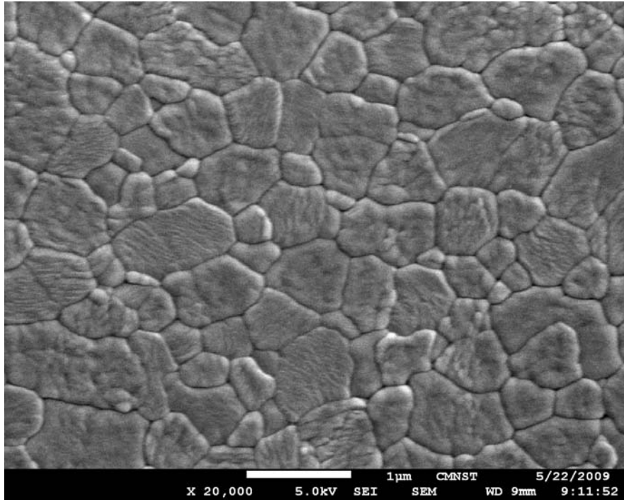
Fig. 6 - SEM of Y-TZP specimen before impact by solid particles at 90° at pH 7 after 20 h (Section 3)
