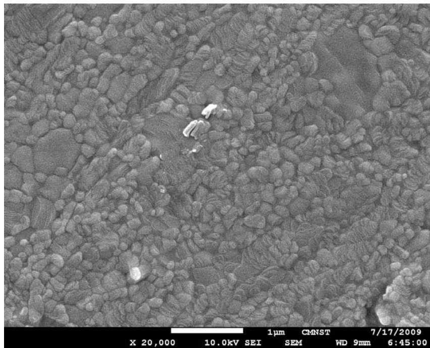
Fig. 9 - SEM observation of Y-TZP after impact by solid particles at 15° after 20h (Section 3)
