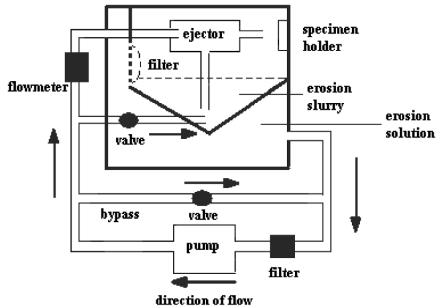
Fig. 1(a) Impinging jet particle slurry erosion apparatus
