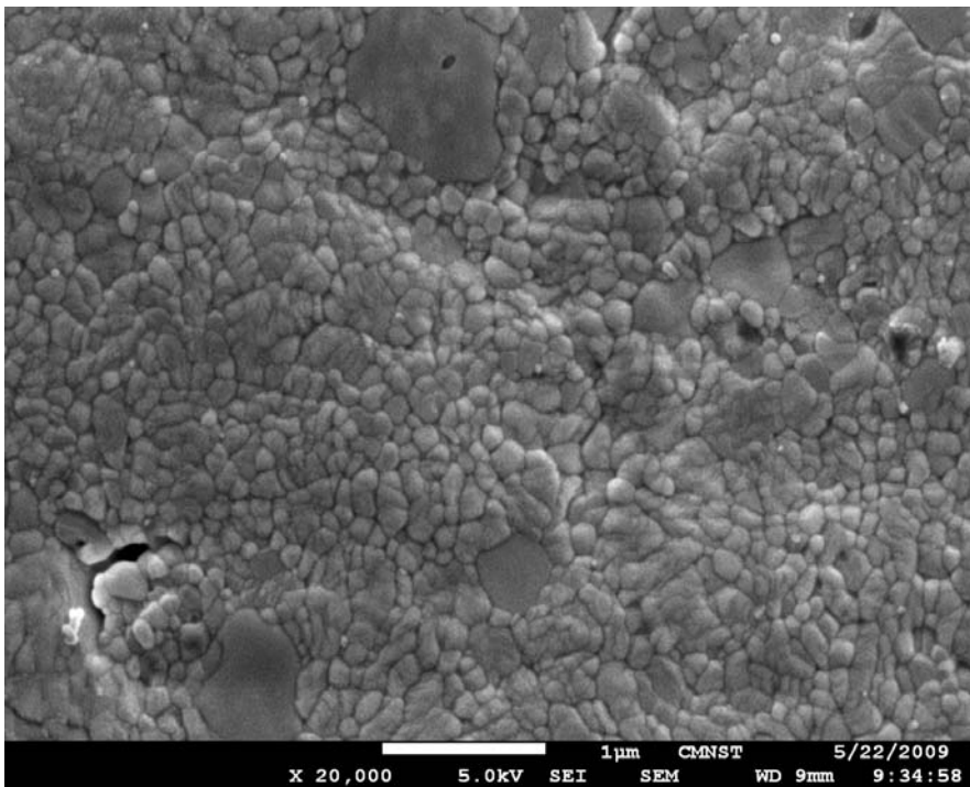
Fig. 7 - SEM of Y-TZP specimen after impact by solid particles at 90° at pH 7 after 20 h (Section 3)
