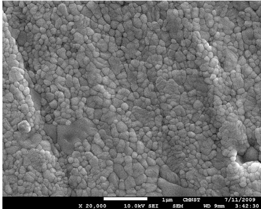
Fig. 10 - SEM observation of Y-TZP specimen after 30° erosion test
