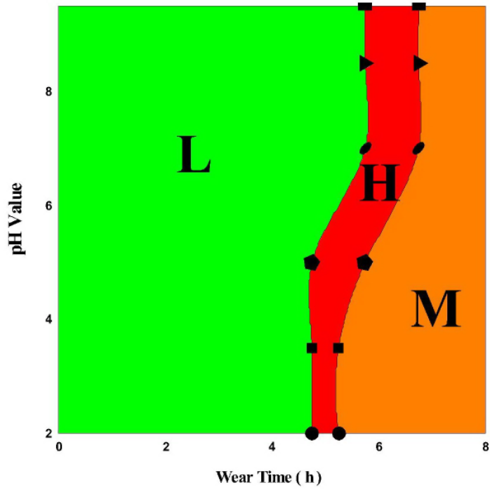
Fig. 20 - Wear rate map at 15° (Green: Low, Orange: Medium, Red: High)
