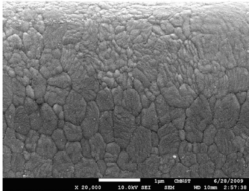
Fig. 8 - SEM observation of a cross-section of Y-TZP specimen after impact by solid particles at 60° after 20h (Section 3) at pH7.
