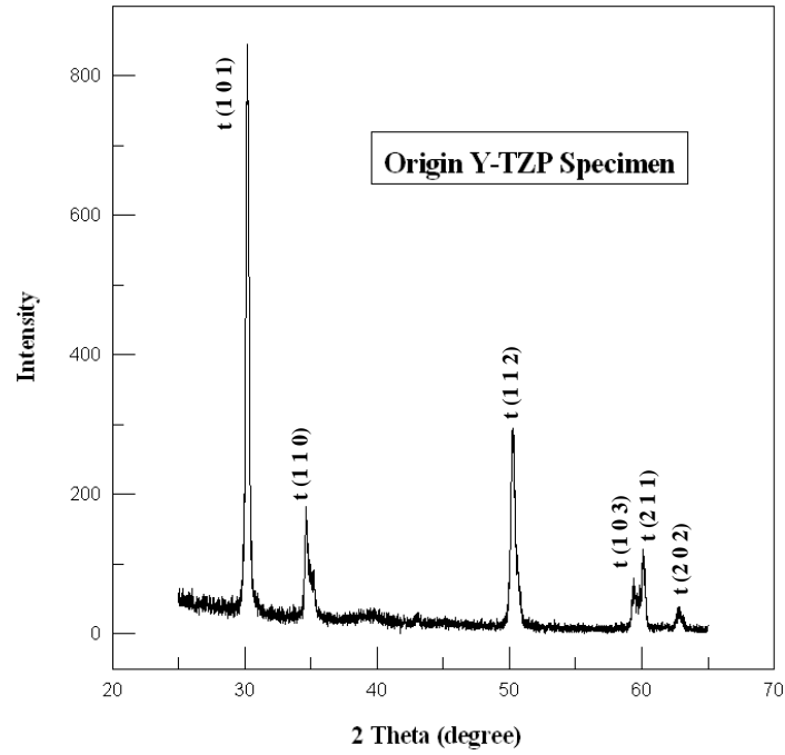
Fig. 2 - XRD analysis of the original Y-TZP specimen
