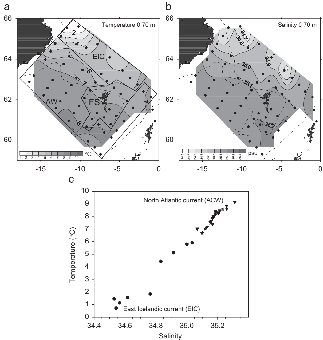
Fig. 2. (a) Temperature (°C) and (b) salinity distributions averaged over the upper 70 m of the water column, (c) T/S plot showing mixing of the two major water masses: the cold, less saline East Icelandic Current (EIC) and the warm saline North Atlantic Current Water (ACW). Areas of EIC, AW and FS are outlined in panel (a). The different symbols show the division into areas (see Section 3.5) based on water characteristics: (●) EIC, (▼) AW, (☆) FS (Table 1).
