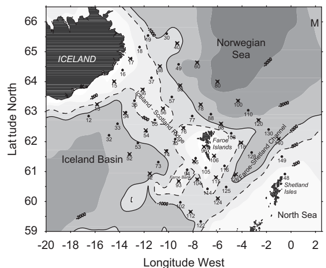
Fig. 1. R/V Dana , cruise 6/97, 4–19 April 1997. Sampling grid over the Iceland–Scotland Ridge. Bullets indicate stations sampled for CTD, Calanus finmarchicus abundance and C. finmarchicus wax ester content, while crosses indicate stations where primary and secondary production, gut fluorescence and seston fatty acid composition were measured. M: approximate location of weather ship M.
