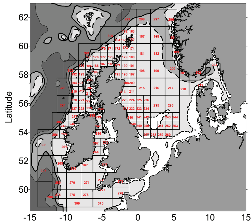
Figure 3.2 Configuration of upper and lower layer boxes in the "sc278" ERSEM model.
