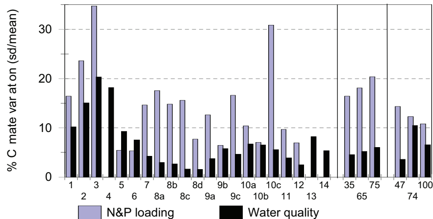
Figure 4.9 Climate variability, expressed as the standard deviation as a percentage of the mean, for reference loadings and model run results using 1984, 1987 and 1990 environmental forcing. The water quality results were a weighted average of the percentage standard deviations for each of the seven assessment criteria.
