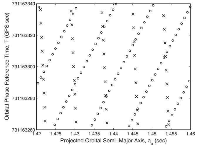
FIG. 10. Here we show a small section ( \approx 1/50 th) of the total orbital parameter space. The crosses and circles represent template locations used to search the L1 and H1 data sets, respectively. This particular template bank was generated for a maximum search frequency of 465 Hz. Note that the templates are not uniformly spaced in the (a_p, \bar{T}) parameter space, although they appear nearly so in the limited region shown here.
