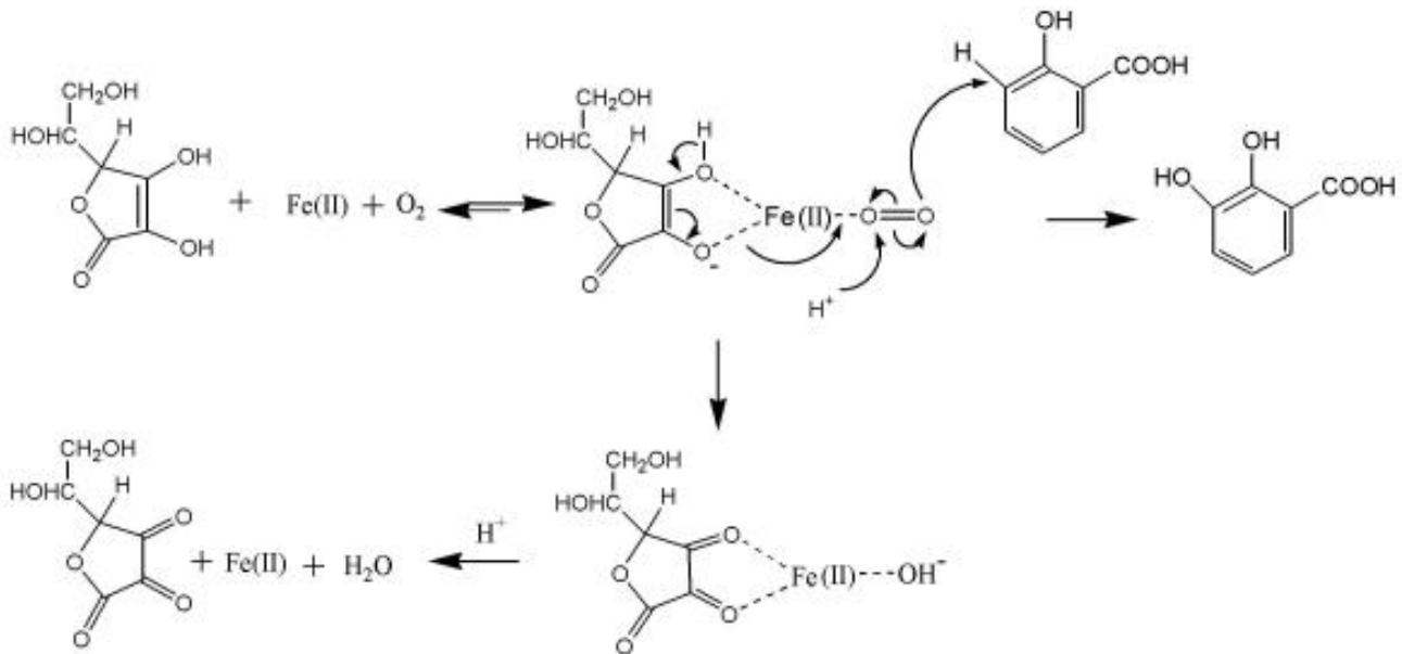
Figure 1 Proposed mechanism for the generation of \text{H}_2\text{O}_2 via the oxidation of ascorbic acid
