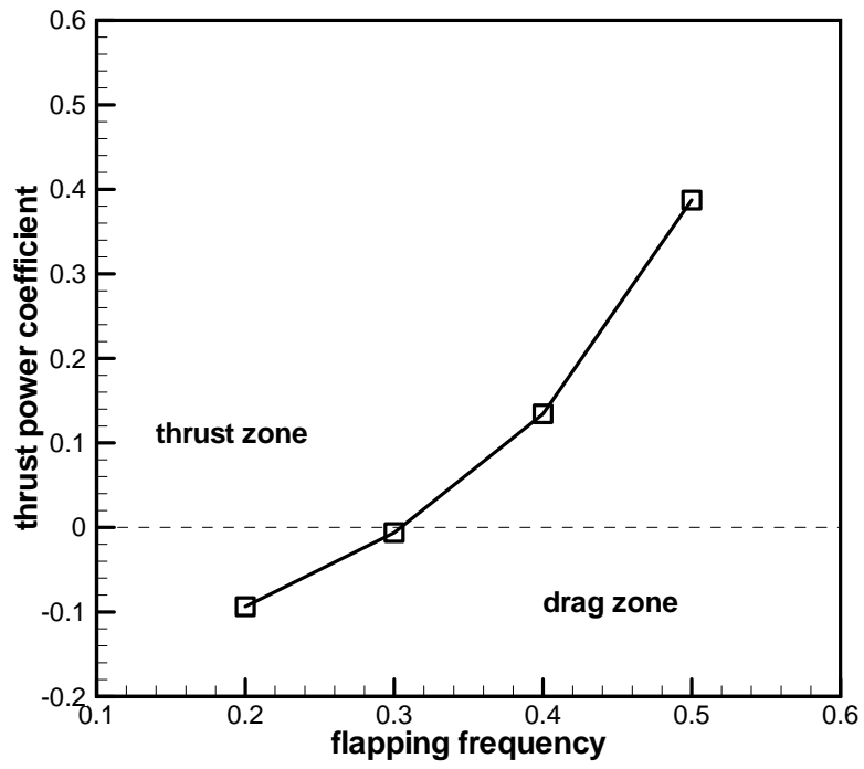
Fig. 19 Effect of flapping frequency on thrust power coefficient
