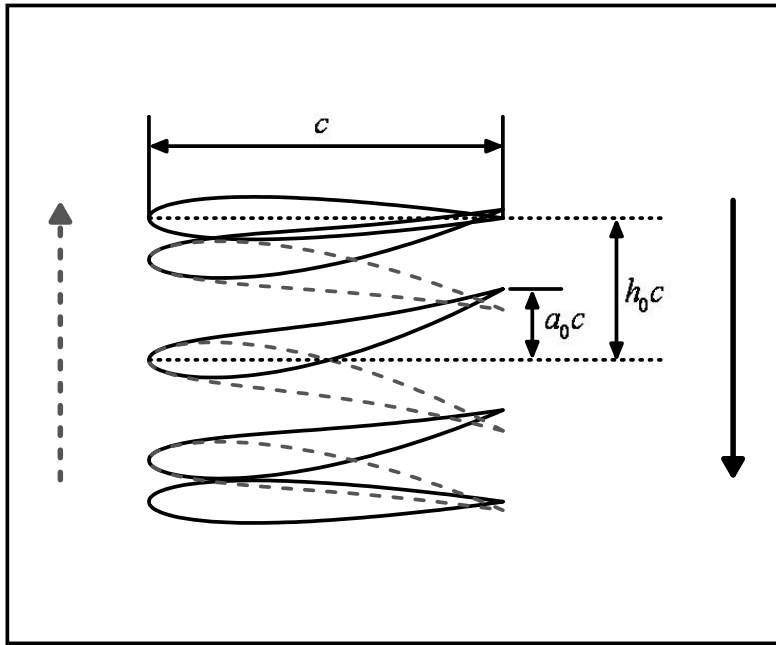
Fig. 13 Plunge and deflection motion of a single flexible airfoil (solid line: downstroke motion; dashed line: upstroke motion)
