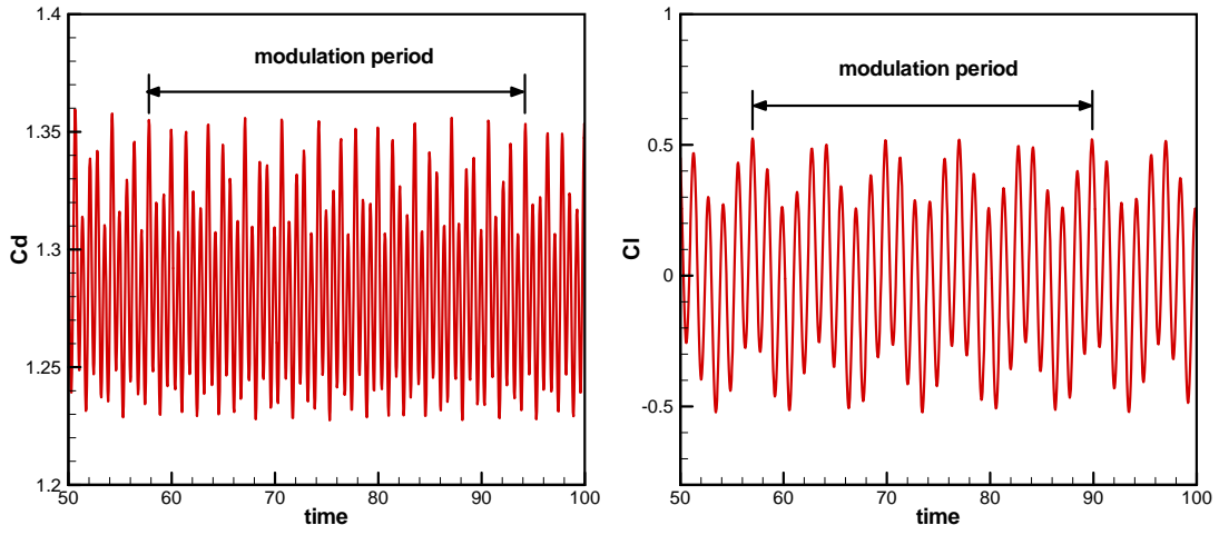
(a) St_f = 0.7
