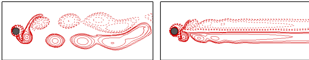
(c) St_f = 0.16
