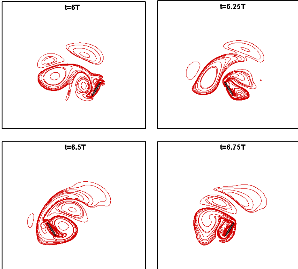
Fig. 11 Vorticity contours in one cycle for \phi = -\pi/4
