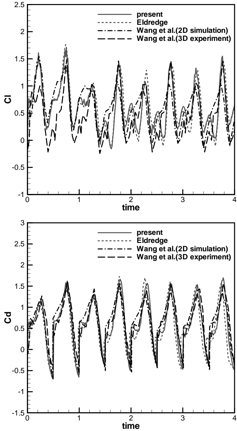
Fig. 10 Time histories of lift and drag coefficients for \phi = \pi/4
