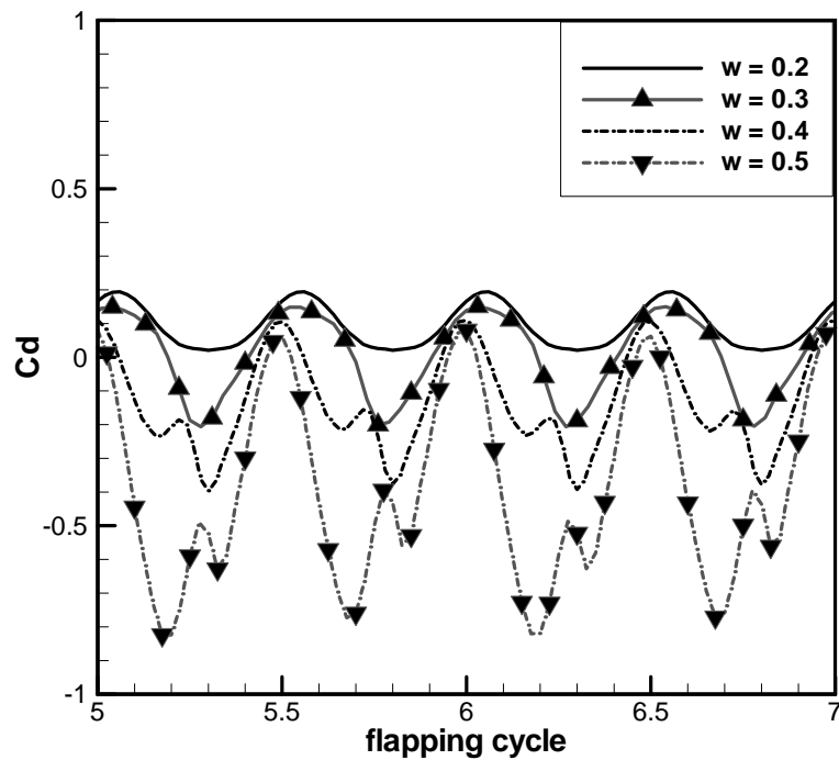
Fig. 18 The evolution of drag coefficients with different frequencies
