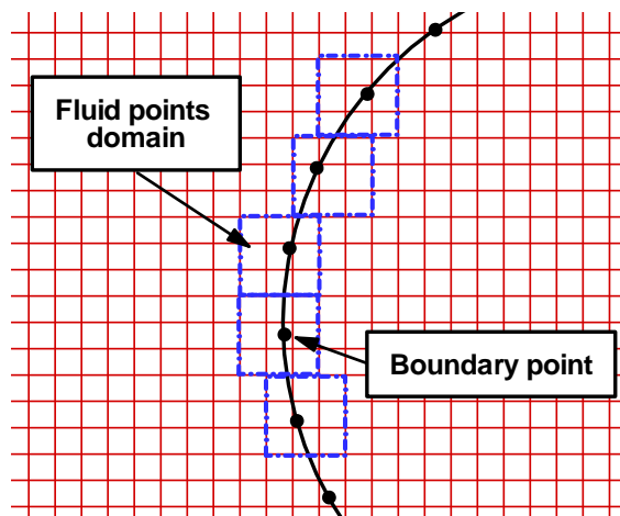
Fig. 1 Configuration of boundary points and their surrounding fluid points
