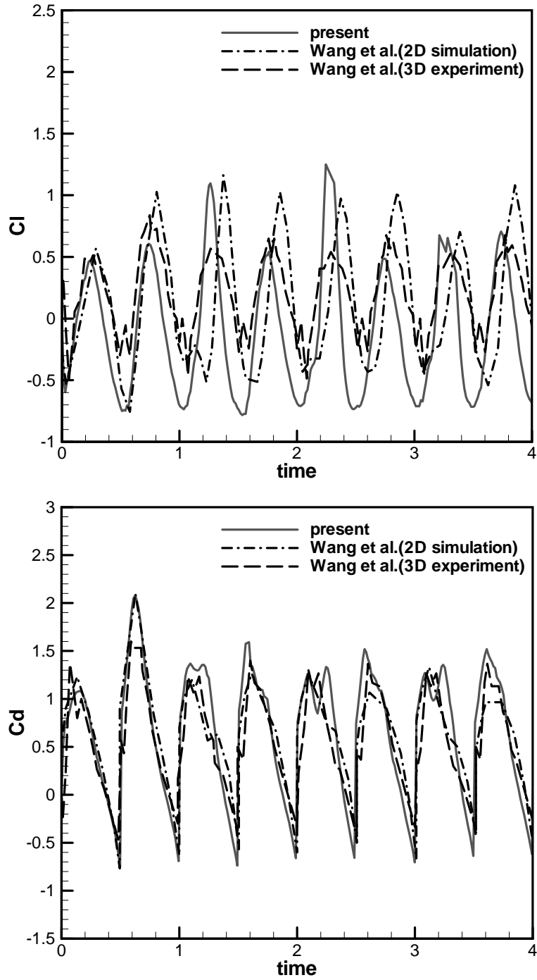
Fig. 12 Time histories of lift and drag coefficients for \phi = -\pi/4
