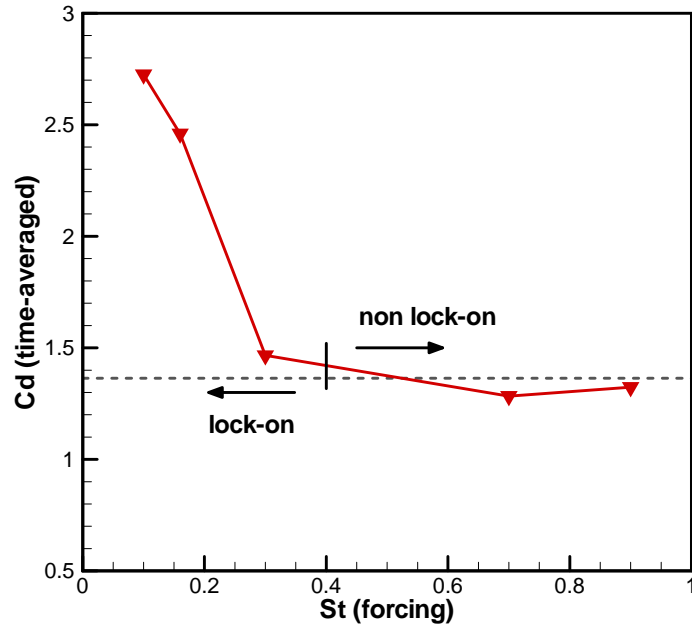
(a) time-averaged drag coefficients (dash line: the value for stationary cylinder case)
