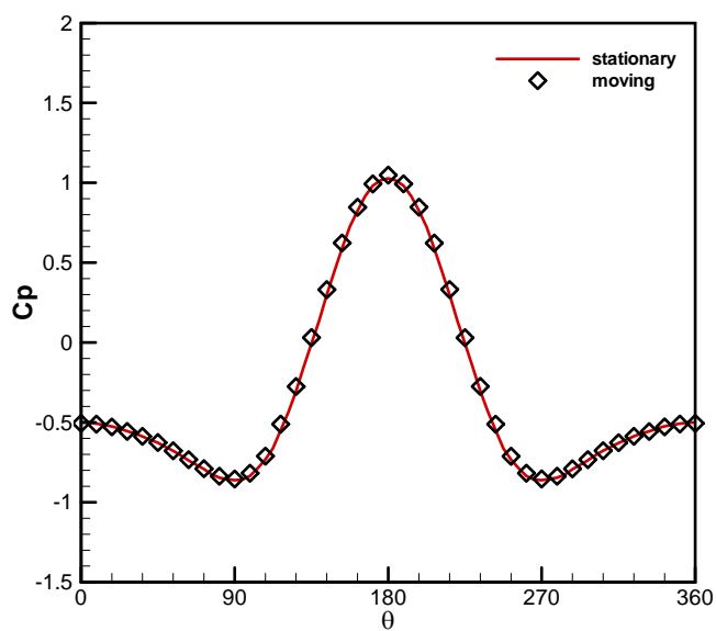
Fig. 4 Pressure distribution on the surface of cylinder at Re = 40
