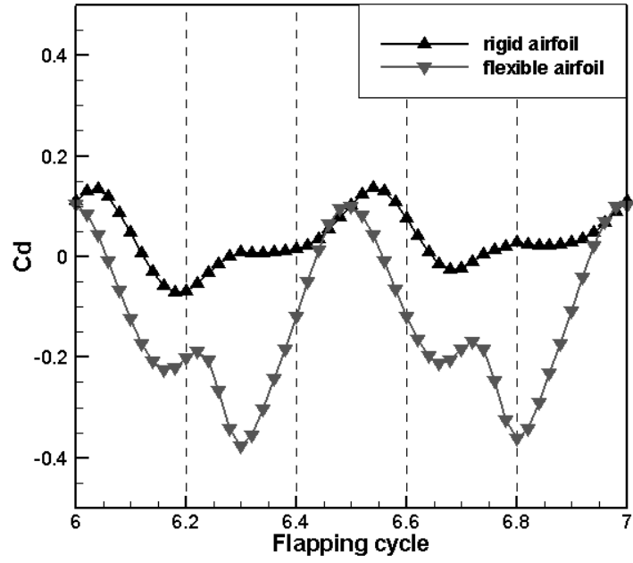
Fig. 15 The evolution of drag coefficients for rigid and flexible airfoils
