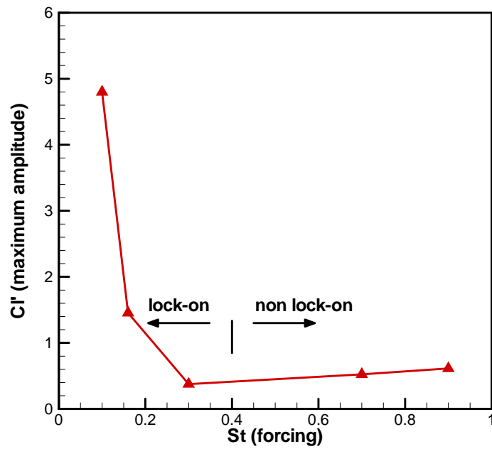
(b) maximum amplitude of the lift coefficient fluctuation
