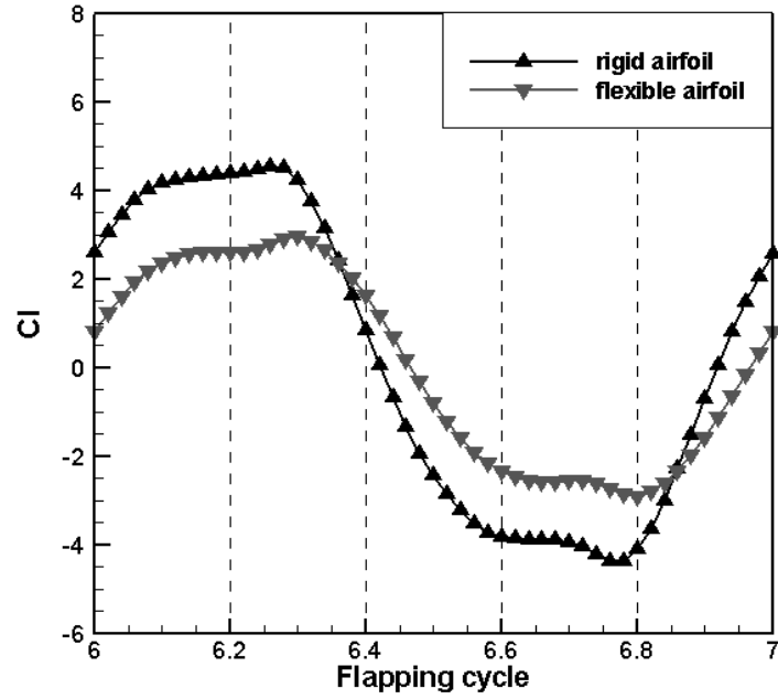
Fig. 17 The evolution of lift coefficients for rigid and flexible airfoils
