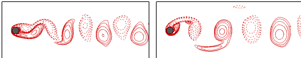
(a) stationary
