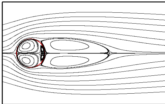
Fig. 2 Streamlines for flow over a stationary cylinder at Re = 40
