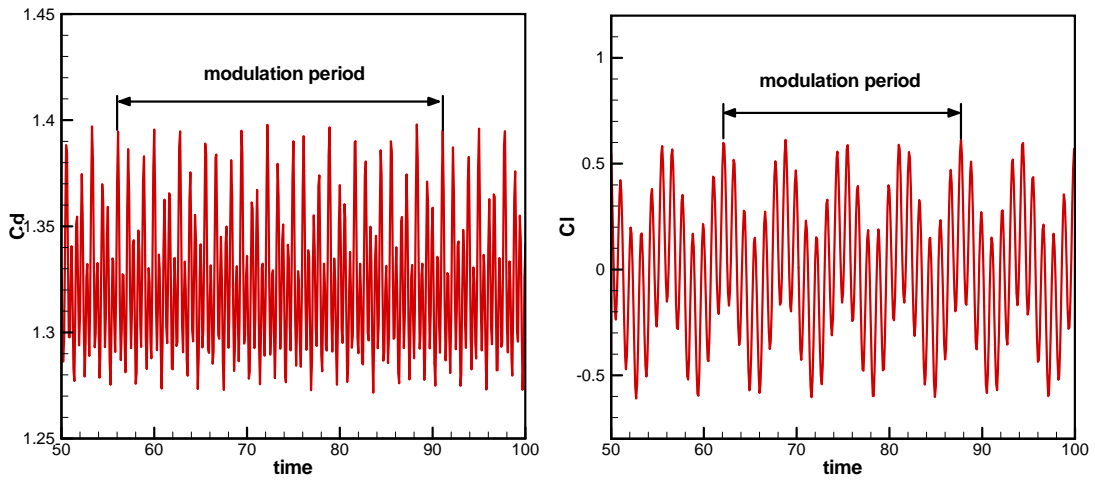
(b) St_f = 0.9
