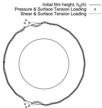
Figure 17: Comparison of film height ( 100\times actual) of present results under shear and surface-tension loading with those under pressure and surface-tension loading at t = 6.9 \times 10^{-3} s, where the incident wind acts from the left.
