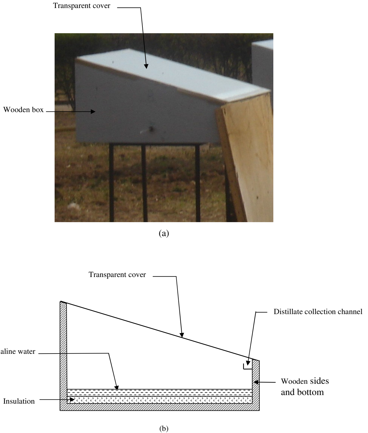
Fig.1: a) Perspective view of a single-slope conventional solar still placed on a table during outdoor testing at the Malawi Polytechnic ( 15^{\circ} 48' S, 35^{\circ} 02' E ), and b) cross-section of the still.
