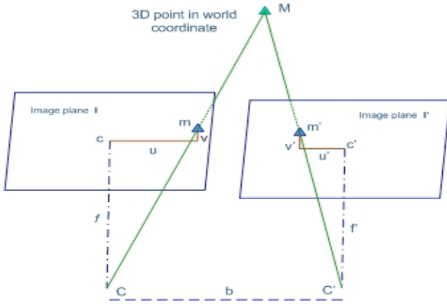
Figure 3 - Disparity estimation using Stereo-pair images
