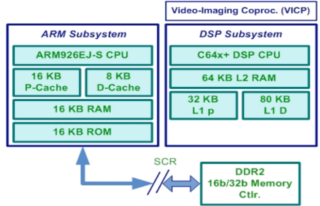
Figure 4 - DM6446 Dual core Architecture
