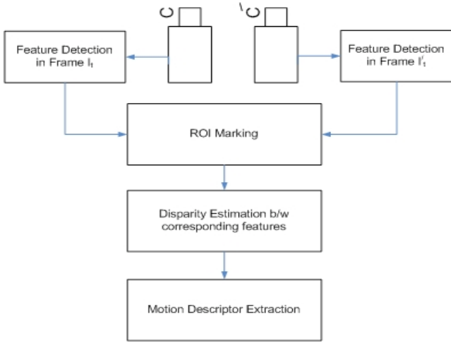
Figure 1 – Block diagram of motion descriptor extraction using stereo-pair footage
