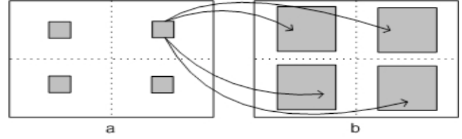
Figure 2 - Stereo frames (a) 4-blocks with search windows of 60x60 (b) showing reference frame with search windows of 150x150
