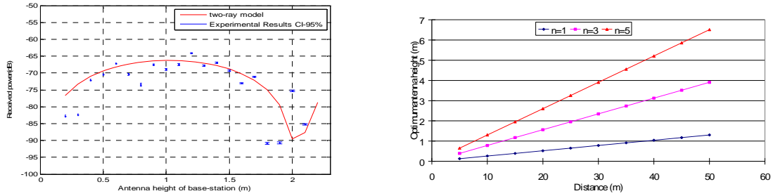
Figure 3: (a) Optimum antenna height at base station; (b) optimum antenna height ( n=1, 2, 5 ).
