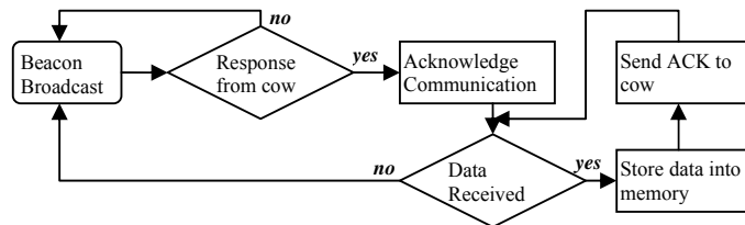
Figure 6: Data collector flow chart diagram
