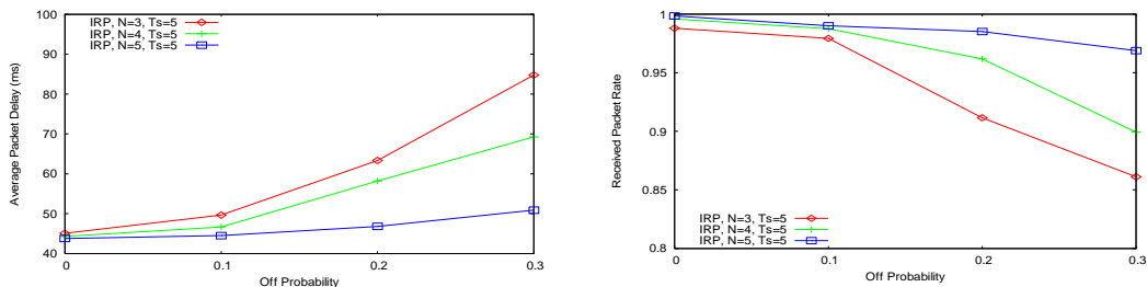
Figure 5: (a) average packet delay; (b) received packet rate.
