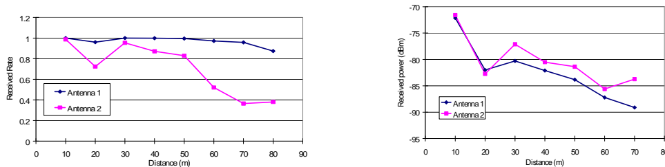
Figure 2: (a) Antenna 1 faces towards base station vs. Antenna 2 faces away from base station; (b) Antenna 1 faces to right perpendicular angle vs. Antenna 2 faces left perpendicular angle.
