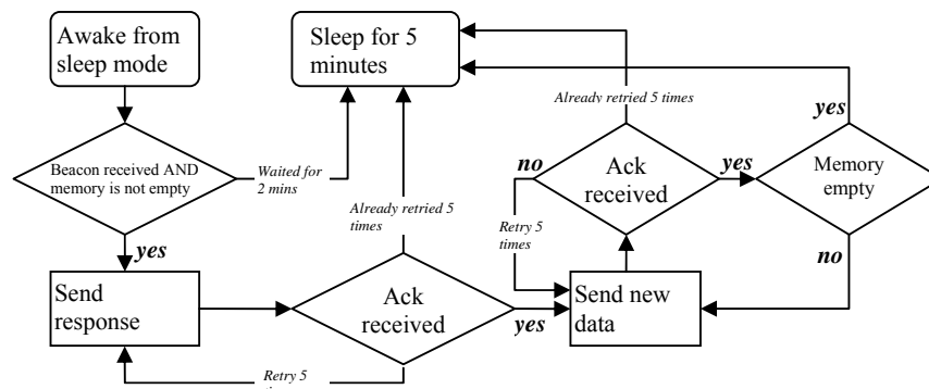
Figure 7: Sensor node operational protocol.
