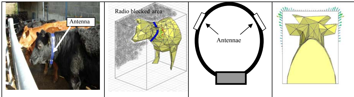
Figure 1: (a) Antenna location on collar; (b) Radio shadow cast by animal; (c) enhanced collar design with two antennas; (d) RF propagation from redesigned collar.
