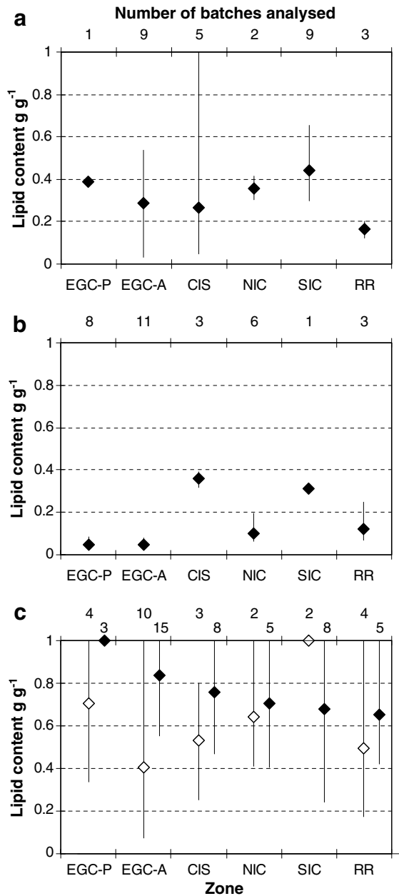
Fig. 13. Mean and range of lipid content (wax ester plus tri acyl glyceride; \text{g (g dry weight)}^{-1} ) of C. finmarchicus , averaged over each zone for each survey. (a) Stage C5 during survey D258, (b) stage C6 females during survey D262, (c) stage c5 during survey D264. Numbers along the upper x axis of each panel indicate the batches of specimens analysed from each zone. For survey D264, animals collected above and below the 200 m depth horizon are discriminated by the symbols (open symbols shallower than 200 m, filled symbols deeper than 200 m; batches of specimens analysed: upper row shallower than 200 m, lower row deeper than 200 m).
