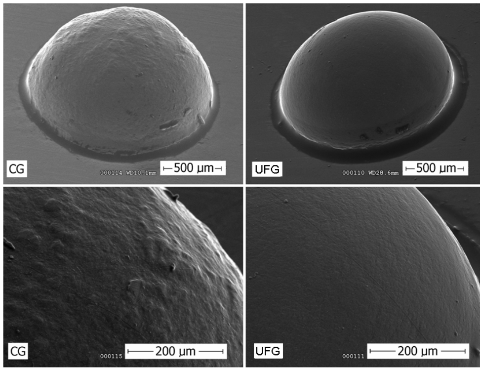
Fig. 4. SEM pictures of the dome part of a microformed component made of CG and UFG Al1070. 24
