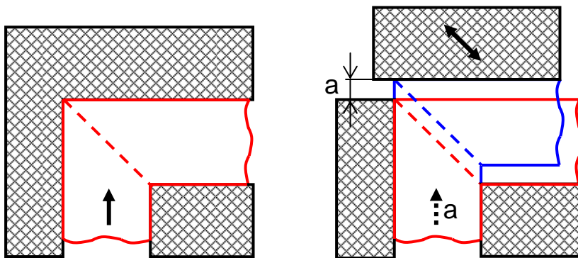
Fig. 3. Schematics of classical ECAP and I-ECAP. 19
