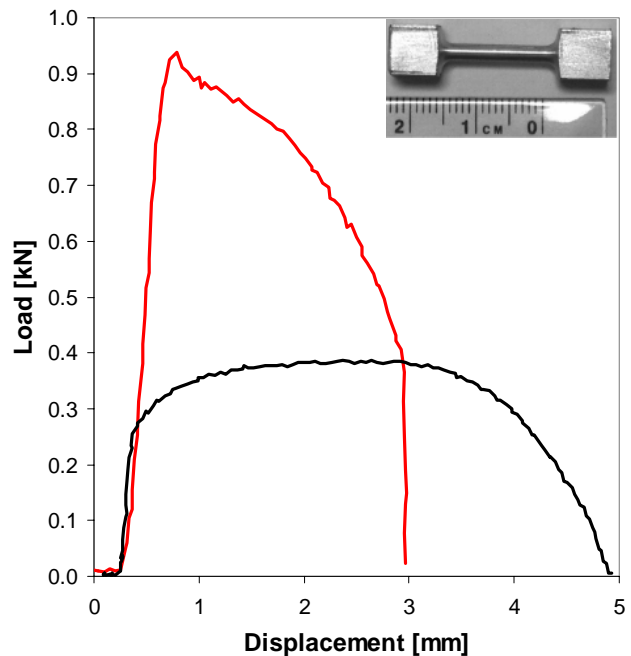
Fig. 2. Tensile behaviour of Al 1070 in initial state and after 8 passes of I-ECAP. 19
