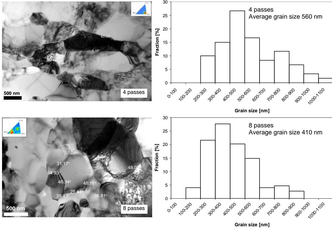
Fig. 1 TEM images and grain size distribution in Al 1070 subjected to 4 and 8 passes of I-ECAP. 19
