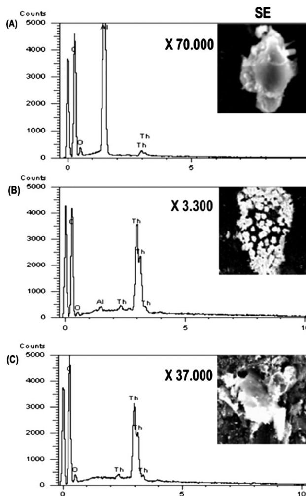
Fig. 1 ED X-ray spectra and secondary electron mappings from the (A) outer, (B) intermediate, and (C) inner regions of a non-pyrolytic graphite platform containing 100 µg each of aluminium and thorium nitrates heated to 2000 °C.
