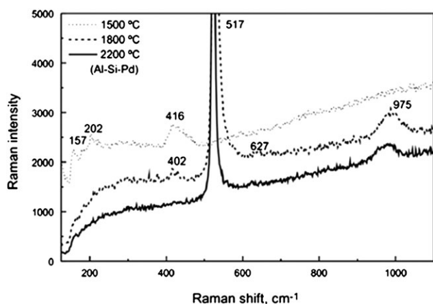
Fig. 5 Raman spectra of pyrolytic graphite platforms containing 100 µg each of aluminium nitrate and palladium chloride, and 100 µg silicon, heated to 1500, 1800 and 2200 °C.
