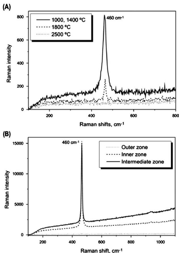
Fig. 2 Raman spectra of (A) 100\text{ }\mu\text{g} of thorium (as nitrate) on pyrolytic graphite platforms heated to different temperatures and (B) 100\text{ }\mu\text{g} each of aluminium and thorium nitrates on three different locations of a non-pyrolytic graphite platform heated to 1800\text{ }^\circ\text{C} .
