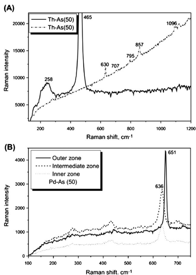
Fig. 7 Raman spectra from different locations of pyrolytic graphite platforms containing (A) 100 µg of thorium nitrate and 500 ng arsenic and (B) 100 µg palladium chloride and 500 ng arsenic, heated to 1200 °C.
