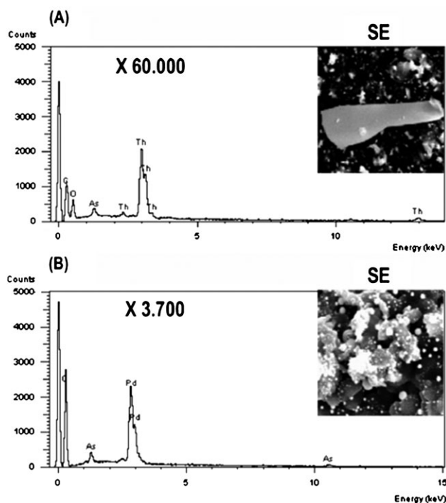
Fig. 6 ED X-ray spectra of pyrolytic graphite platforms containing (A) 100 µg of thorium nitrate and 500 ng of arsenic and (B) 100 µg palladium chloride and 500 ng arsenic, heated to 1200 °C.
