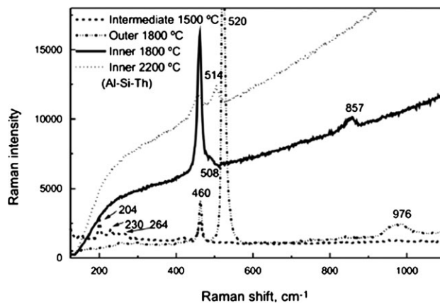
Fig. 4 Raman spectra of three different locations of pyrolytic graphite platforms containing 100\text{ }\mu\text{g} each of aluminium and thorium nitrates and 100\text{ }\mu\text{g} silicon, heated to 1500 , 1800 and 2200\text{ }^\circ\text{C} .
