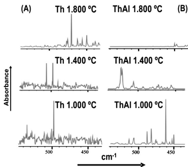
Fig. 3 FT-IR absorbance spectra of the solid residue from a large area of a graphite platform containing (A) 100\text{ }\mu\text{g} of thorium nitrate and (B) 100\text{ }\mu\text{g} each of aluminium and thorium nitrates heated to 1000\text{ }^\circ\text{C} , 1400\text{ }^\circ\text{C} and 1800\text{ }^\circ\text{C} .
