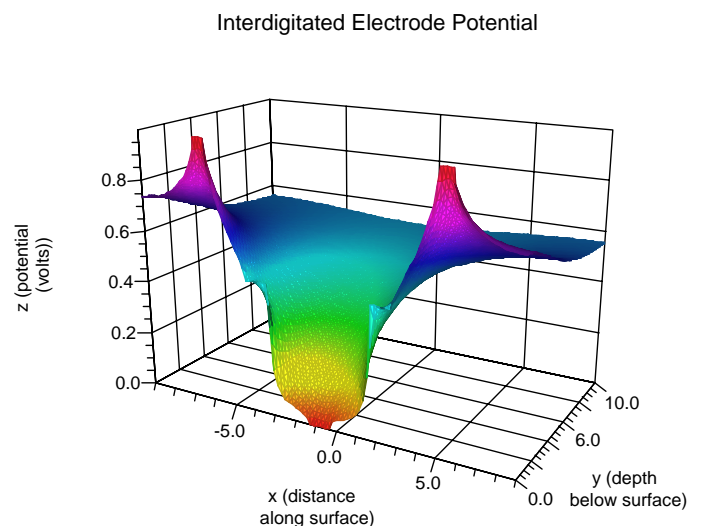
Fig. 2. Inter-digitated electrode potential profile showing field penetration to a depth of several millimetres below the surface.
