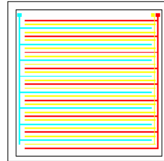
Fig. 1. Inter-digitated electrode structure allowing single sided low frequency measurements of a GRP structure.
