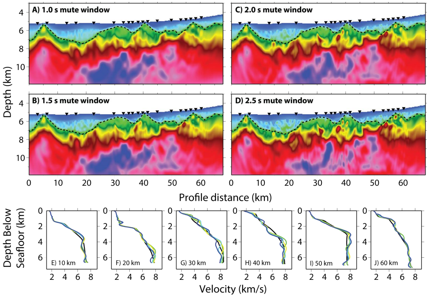
Figure 7: Inversion models for varying mute windows of A) 1.0 s B) 1.5 s C) 2.0 s D) 2.5 s. Black upturned triangles indicate the locations of utilised instruments, black dashed line indicates the base of post-rift sediments. Vertical exaggeration is 3.2. E-J) 1D velocity profiles through the resulting models, below the seafloor, at set profile distances (10, 20, 30, 40, 50 and 60 km, respectively). Line colours are black: starting model, green: 1.0 s, yellow: 1.5 s, light blue: 2.0 s, blue: 2.5 s.
