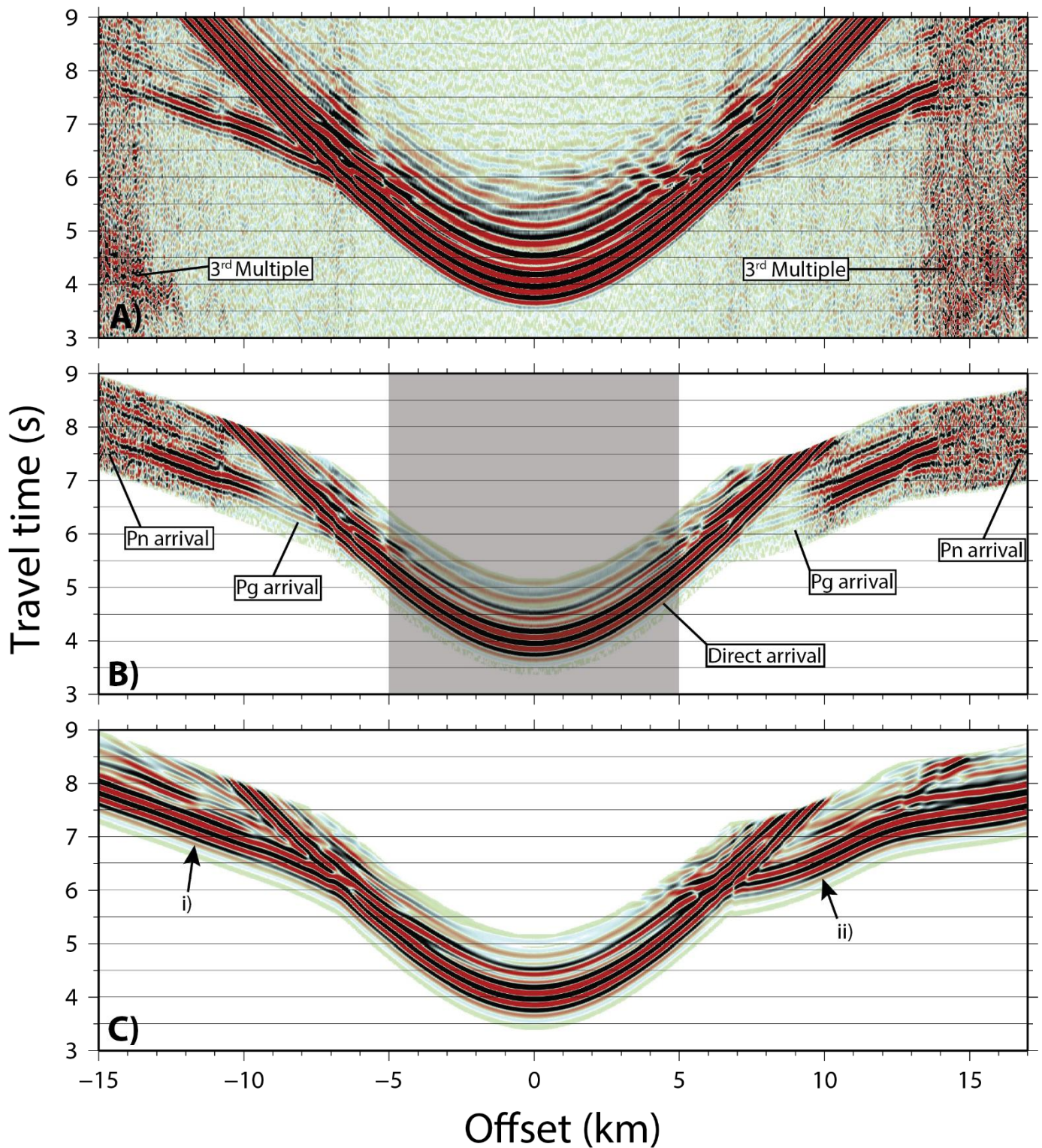
Figure 2: A) Example receiver gather from OBS 46, filtered with an Ormsby band-pass comprised of corner frequencies 2-3-4.5-6.5 Hz. The 3 rd multiple from the previous seismic shot is indicated. B) Same receiver gather as in A), windowed 1.8 s after the first arrival for input into the inversion process. Grey area indicates data excluded from the inversion. Identified seismic phases are indicated. C) Synthetic receiver gather for OBS46 generated using the starting velocity model in Fig 4A.
