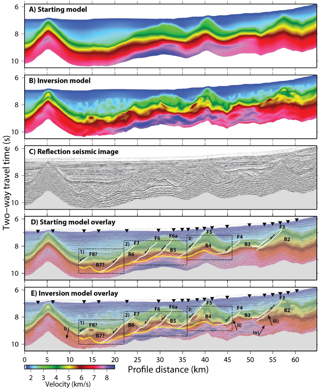
Figure 14: Comparison of large scale features with seismic reflection imaging. A) Starting velocity model B) Final FWI velocity model C) Kirchhoff pre-stack time-migrated multichannel seismic image of inline 420. D) Reflection image overlain with starting velocity model. E) Reflection image overlain with FWI velocity model. White lines indicate the
