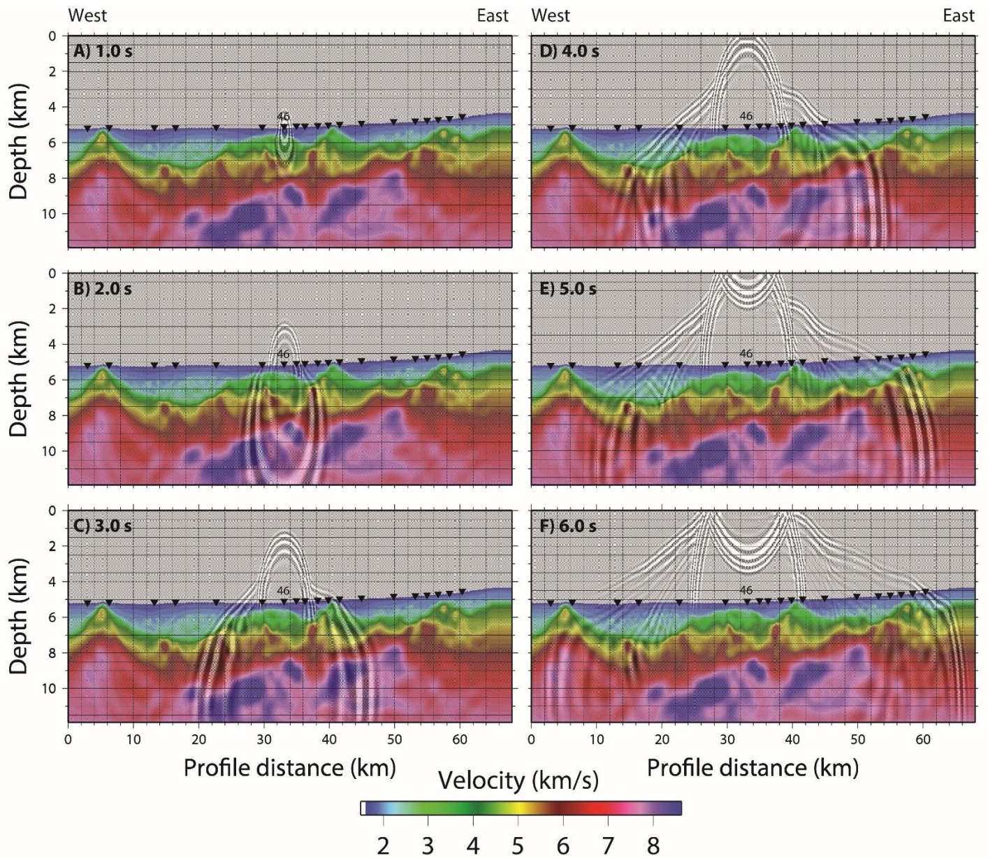
Figure 9: Propagation of the derived source wavelet through the final inversion model, originating at OBS46, at discrete times: A) 1.0 s, B) 2.0 s, C) 3.0 s, D) 4.0 s, E) 5.0 s, F) 6.0 s. Black upturned triangles indicate the locations of utilised instruments. Vertical exaggeration is 3.2.
