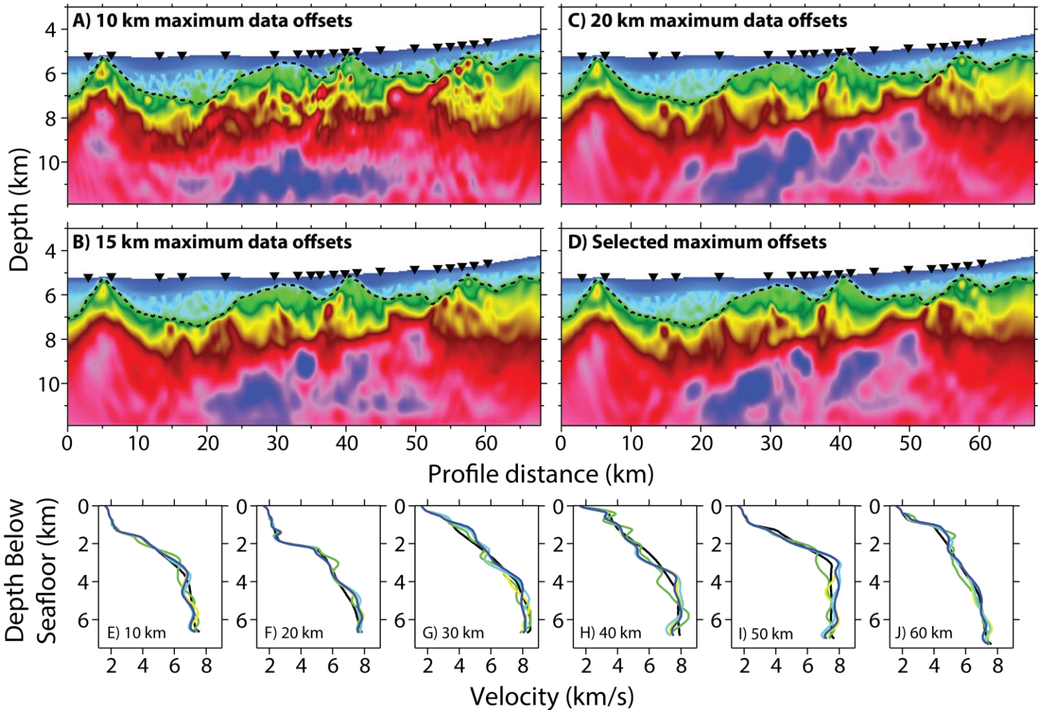
Figure 6: Inversion models for maximum data offsets of A) 10 km B) 15 km C) 20 km D) Instrument specific offsets. Black upturned triangles indicate the locations of utilised instruments, black dashed line indicates the base of post-rift sediments. Vertical exaggeration is 3.2. E-J) 1D velocity profiles through the resulting models, below the seafloor, at set profile distances (10, 20, 30, 40, 50 and 60 km, respectively). Line colours are black: starting model, green: 10 km data offsets, yellow: 15 km data offsets, light blue: 20 km data offsets, blue: instrument specific data offsets.
