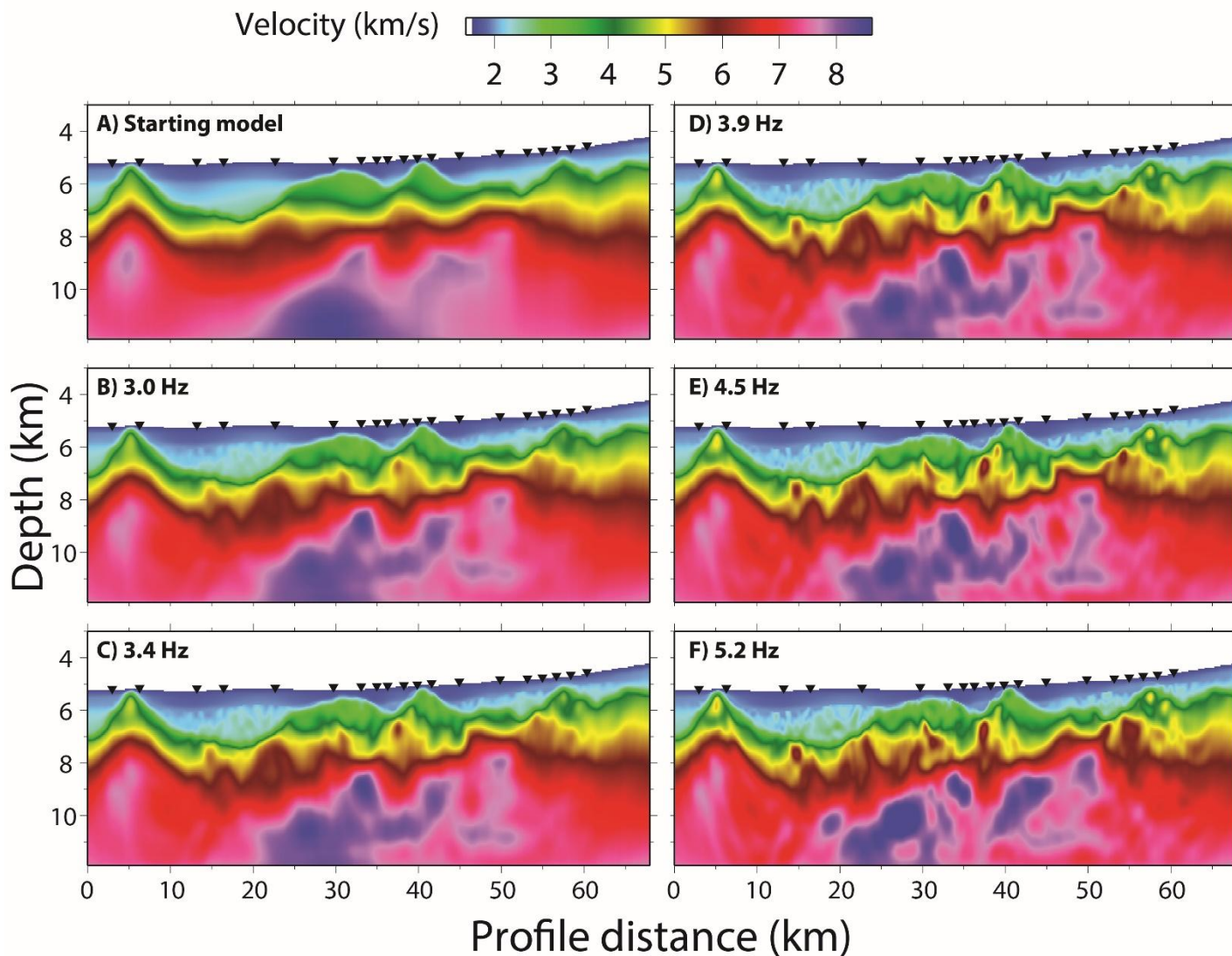
Figure 4: A) Starting velocity model input to the FWI. Results of the iterative FWI process for low-pass filter frequencies of: B) 3.0 Hz; C) 3.4 Hz; D) 3.9 Hz; E) 4.5 Hz and F) 5.2 Hz. Black upturned triangles indicate the locations of utilised instruments. Vertical exaggeration is 3.2.
