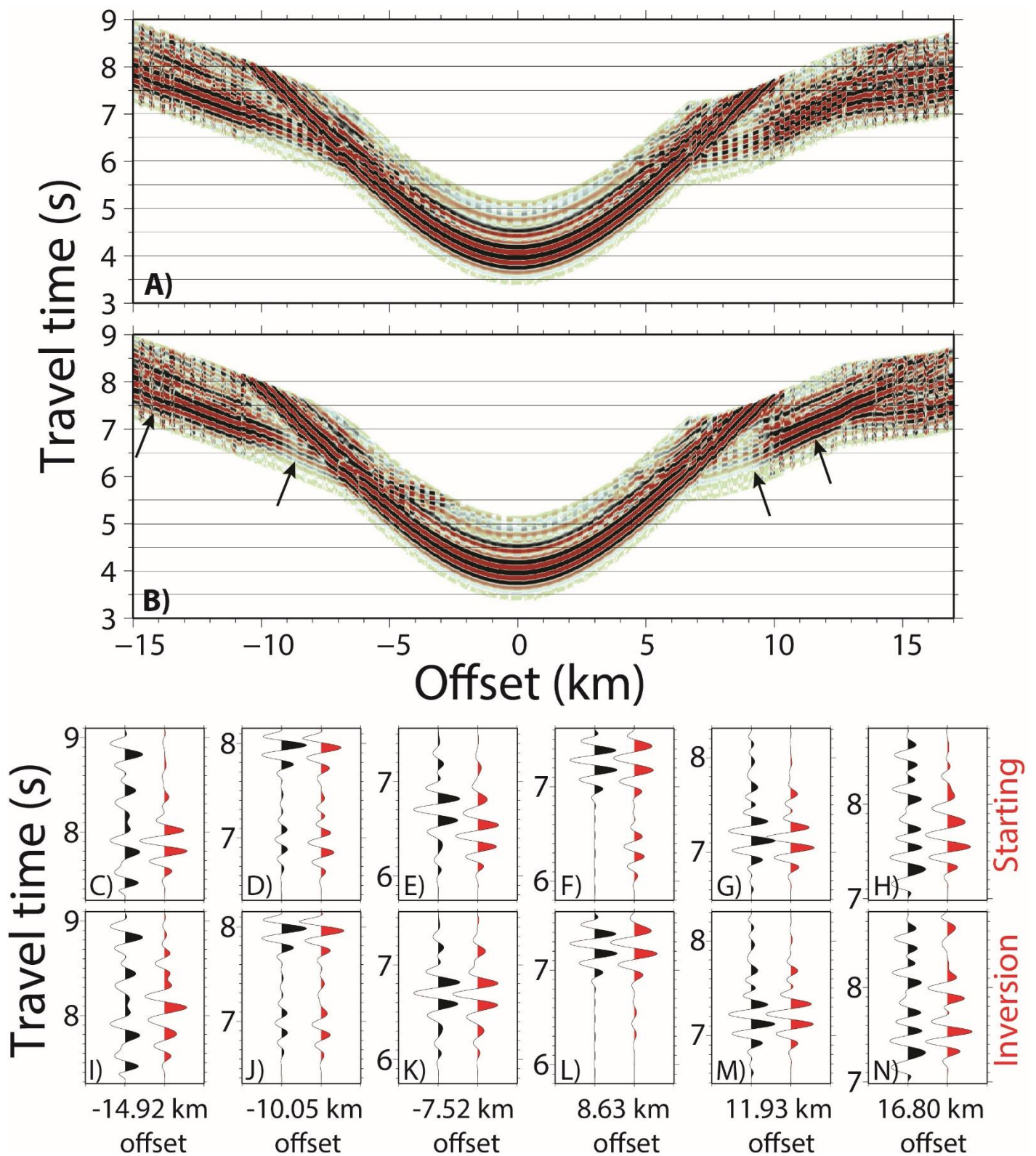
Figure 11: OBS 46. A) Observed data interleaved with synthetic through the starting model in alternative offset bins of 200 m. B) Observed data interleaved with synthetic through the inversion model in alternative offset bins of 200 m. C-H) Black traces: observed data, red traces: synthetic data through the starting model. I-N) Black traces: observed data, red traces: synthetic data through the FWI model.
