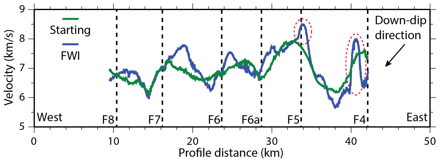
Figure 16: Velocities below the interpreted S-reflector (averaged over a 100 ms window). The green line indicates velocities from the starting velocity model; the blue line indicates velocities from the final FWI velocity model. Vertical dashed lines indicate the locations where interpreted normal faults sole onto the S-reflector. Red dashed ellipses indicate anomalous features of the inversion model.
