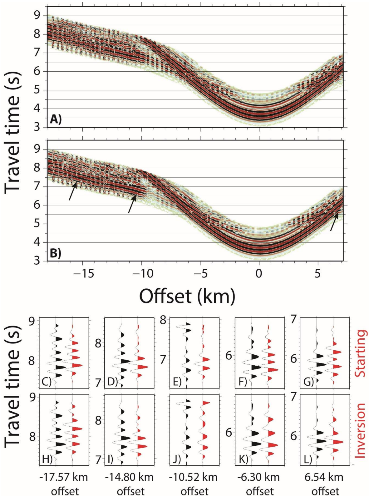
Figure 12: OBS 54. A) Observed data interleaved with synthetic through the starting model in alternative offset bins of 200 m. B) Observed data interleaved with synthetic through the inversion model in alternative offset bins of 200 m. C-G) Black traces: observed data, red traces: synthetic data through the starting model. H-L) Black traces: observed data, red traces: synthetic data through the FWI model.
