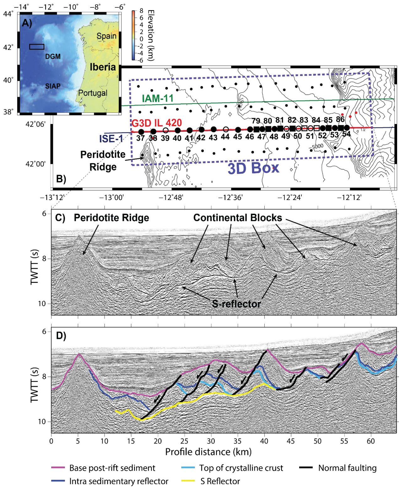
Figure 1: A) Bathymetric map of the Deep Galicia Margin (DGM) and the Southern Iberia Abyssal Plain (SIAP) with the relative location of Fig. 1B (black rectangle). B) Map of the Galicia-3D seismic experiment. Galicia 3-D inline 420 seismic profile is illustrated by a red
