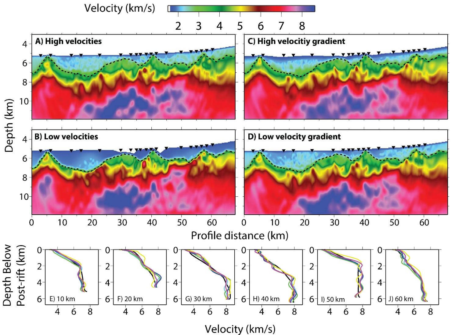
Figure 8: Inversion models for varying starting sediment velocity models, as described in section 3.7: A) High velocities B) Low velocities C) High-velocity gradient D) Low-velocity gradient. Black upturned triangles indicate the locations of utilised instruments, black dashed line indicates the base of post-rift sediments. Vertical exaggeration is 3.2. E-J) 1D velocity profiles through the resulting models, below post-rift sediment, at set profile distances (10, 20, 30, 40, 50 and 60 km, respectively). Line colours are black: starting model, green: high velocities, yellow: low velocities, light blue: high-velocity gradient, blue: low-velocity gradient.
