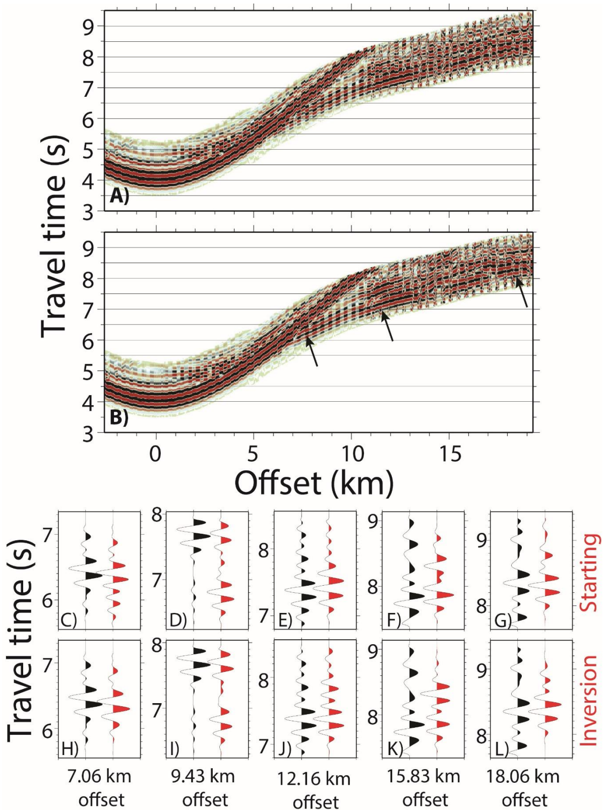
Figure 10: OBS 37. A) Observed data interleaved with synthetic through the starting model in alternative offset bins of 200 m. B) Observed data interleaved with synthetic through the inversion model in alternative offset bins of 200 m. C-G) Black traces: observed data, red traces: synthetic data through the starting model. H-L) Black traces: observed data, red traces: synthetic data through the FWI model.
