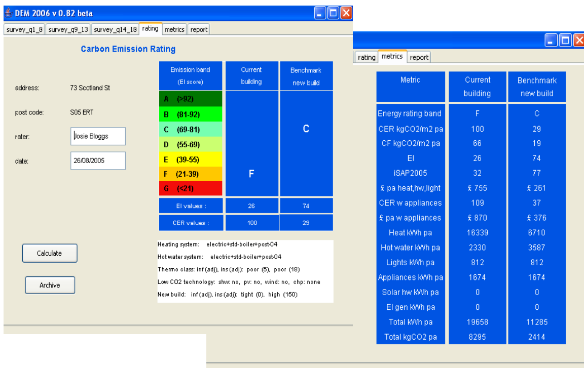
Figure 4: Montage of EDEM outputs.
