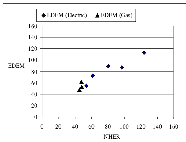
Figure 1: CO 2 emissions (kg /m 2 yr) – EDEM vs. NHER Surveyor.
