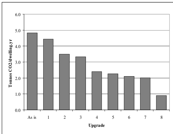
Figure 5: Upgrade impact on carbon footprint.
