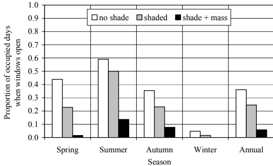
Figure 11 Predicted window opening v. building design option.
