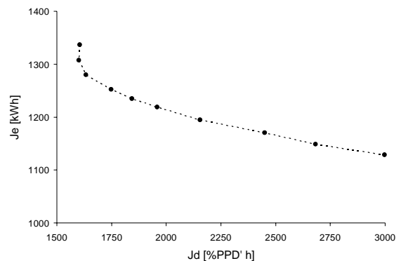
Figure 1: Typical controller performance for different settings. Costs are summed over a given period. Experimental data for that period would yield only 1 point
