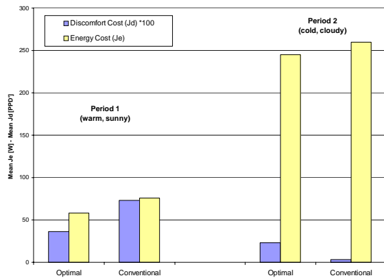
Figure 4: performance comparison based on simulation results, PASSYS test cell
