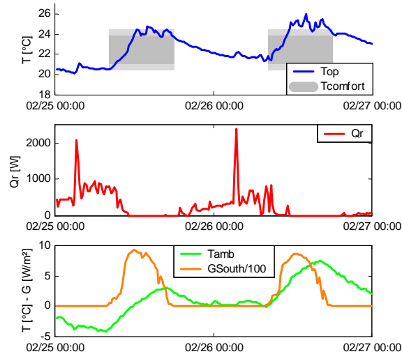
Figure 2: Typical sunny mid-season days, conventional controller
