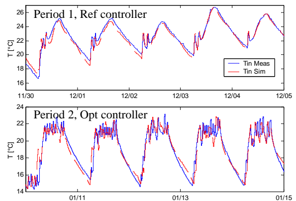
Figure 3: simulated and measured air temperature, PASSYS test cell
