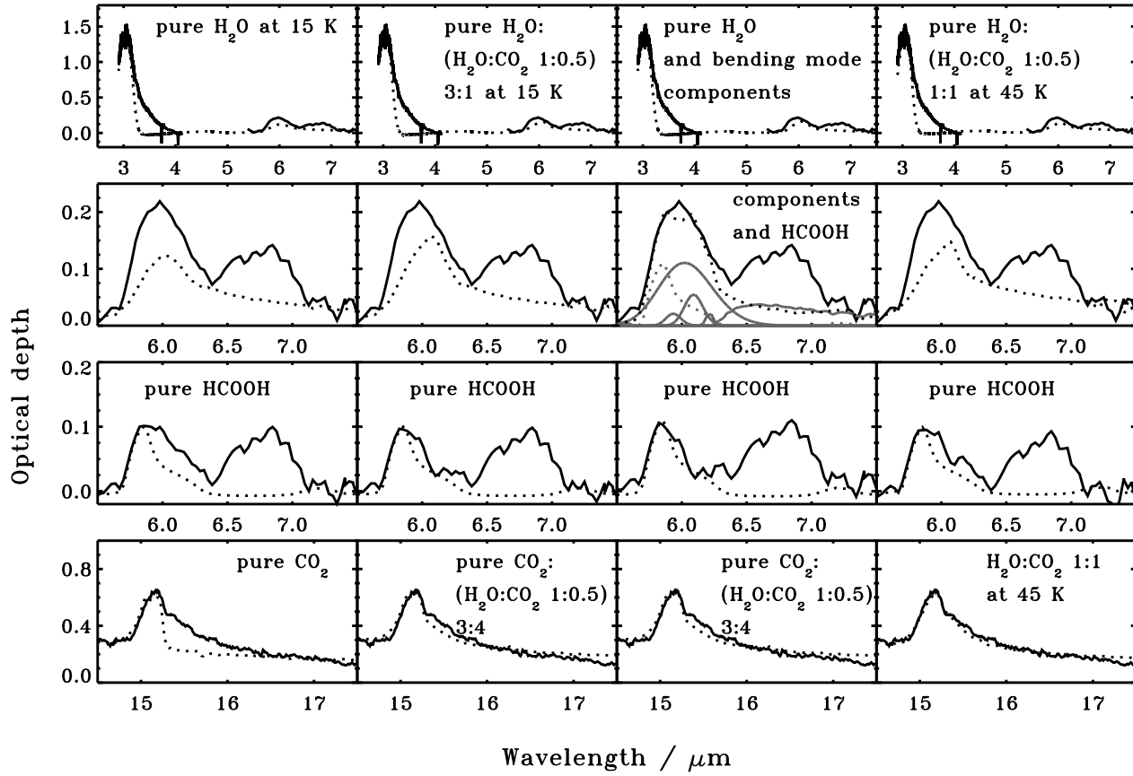
Fig. 11. Spectrum of the YSO B5 IRS1 (solid line) compared with laboratory spectra (dashed) of pure H 2 O and CO 2 at 15 K (first column), a combination of pure H 2 O and the H 2 O:CO 2 1:0.5 ice mixture at 15 K (second column) and 45 K (fourth column) and the derived bending mode components (third column). The silicate feature has been subtracted from the B5:IRS1 spectrum in all plots. In the upper row the spectrum has been fitted with respect to the 3 \mu\text{m} H 2 O stretching band. The effect on the H 2 O bending mode region is shown in the second row. In the third row the H 2 O (mixture) spectra have been subtracted from the star spectrum and the residual is compared with a pure HCOOH spectrum at 15 K. The last row shows the fit to the CO 2 bending mode using the ice mixture derived from the H 2 O modes. The CO 2 peak has been shifted in the laboratory spectra to account for the shift in position between C 16 O 2 and C 18 O 2 used in this study. In the fourth column the spectrum of pure HCOOH was fitted together with the bending mode components to the 6.0 \mu\text{m} band, to achieve an optimal fit while also being consistent with the band strength of the H 2 O stretching mode. The individual components are plotted with a gray line.
