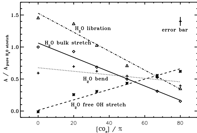
Fig. 4. The band strengths of the four main H 2 O peaks in H 2 O:CO 2 ice mixtures relative to that of the H 2 O stretch in pure H 2 O ice at 15 K. The band strengths of the libration, bend and free OH stretch modes have been multiplied by a factor of 10 to facilitate display. The estimated average error bar of the relative band strengths is shown in the upper right corner.
