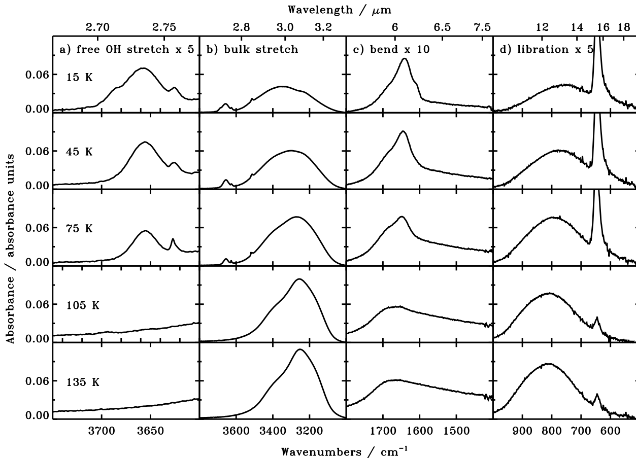
Fig. 6. Temperature dependence of the H 2 O bands in a 1:0.5 H 2 O:CO 2 mixture i.e. 67% H 2 O and 33% CO 2 . Spectra at 4000–400 cm -1 of the four main H 2 O peaks in a 1:0.5 ice mixture with CO 2 at temperatures between 15 and 135 K. Each column contains one of the H 2 O vibrational modes and each row one of the temperatures. a) an expanded view of the H 2 O free OH stretch, b) the H 2 O bulk and free-OH stretch, c) the H 2 O bend and d) H 2 O libration. The spectra of libration, bending and free OH stretch have been scaled, with a scaling factor indicated in the top row.
