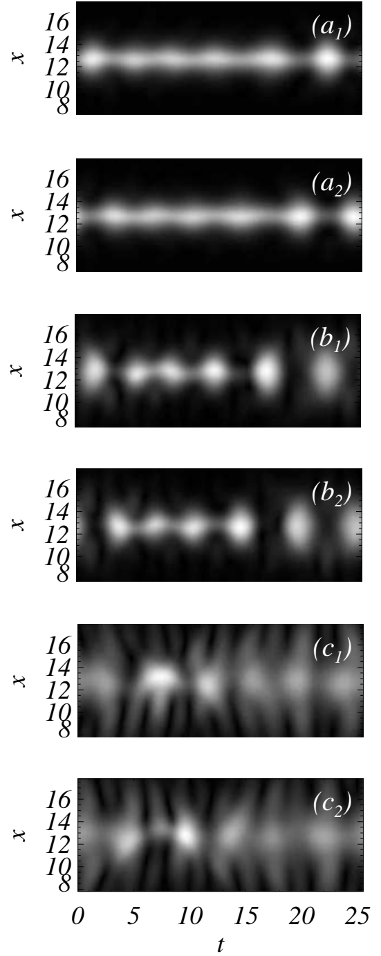
FIG. 9. Development of the anti-phase neck MI for \beta = 7 , \kappa = 1 , \delta = 0 , \gamma = -0.5 . (a 1,2 ) |E_{1,2}| for z = 8.4 ; (b 1,2 ) |E_{1,2}| for z = 10.2 ; (c 1,2 ) |E_{1,2}| for z = 12.6 .
