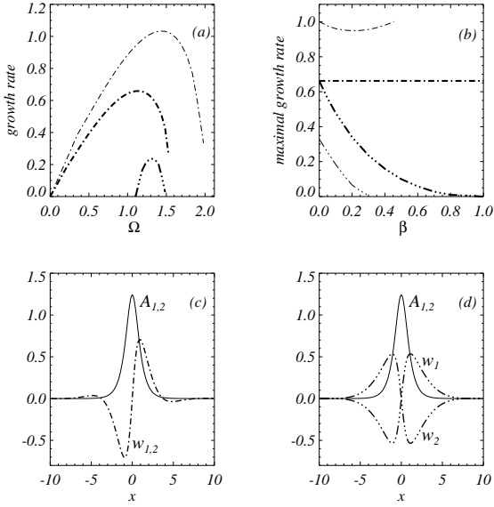
FIG. 4. Instability growth rates, spatial profiles of the solitary solutions and of the unstable eigenmodes for \beta < 1 , \gamma = -0.5 . Dash-dot (dash-dot-dot-dot) lines correspond to the in-phase (anti-phase) snake MI. (a) Growth rates vs \Omega , \beta = 0.3 . Thin (thick) lines correspond to \kappa = 1 , \delta = 0 , Q \simeq 4.04 , Q_u = 0 ( \kappa = 1.155 , \delta = 0.5 , Q \simeq 4.04 , Q_u \simeq 2.18 ). (b) Maximal growth rate vs \beta . Thin (thick) lines correspond to \delta = 0 ( \delta = 0.5 ). (c) Components of the eigenmode corresponding to the in-phase snake MI, \beta = 0.3 , \delta = 0 , \Omega = 1 . (d) Components of the eigenmode corresponding to the anti-phase snake MI, \beta = 0.3 , \delta = 0 , \Omega = 0.92 .
