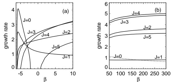
FIG. 4. Growth rates of the maximally unstable eigenmodes vs \beta for one-ring solitary solutions. Dotted line in (b) displays Im\lambda_0 of the J = 0 internal eigenmode marked by Line 1 in Fig. 2. \kappa = 3 .
