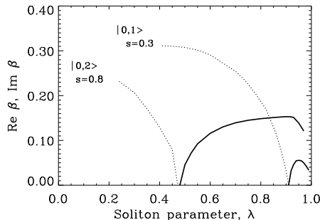
FIG. 3. Instability eigenvalues vs. \lambda for |0,1\rangle and |0,2\rangle solitons; dashed line - \text{Im}\beta , bold line - \text{Re}\beta .
