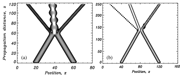
FIG. 5. Collisions of (a) linearly stable |0, 1\rangle solitons at s = 0.8 , \lambda = 0.72 with the relative transverse velocity v = 0.05 , and (b) linearly stable |0, 2\rangle solitons at s = 0.8 , \lambda = 0.35 , with v = 0.09 .
