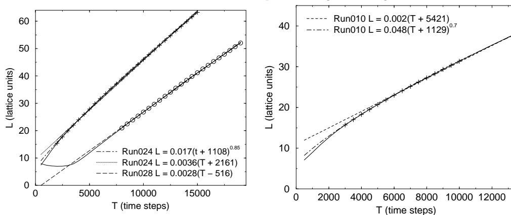
FIGURE 20. Left: 256^3 , L_0 = 36 , Run024 with M = 0.8 compared with Run028 ( M = 0.1 ). Right: Run010, 128^3 , L_0 = 381 , M = 0.5 .
