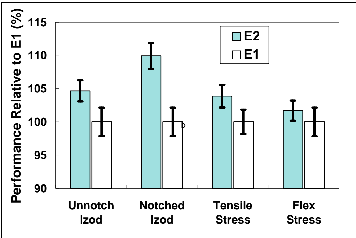
Figure 10: Normalised composite properties
