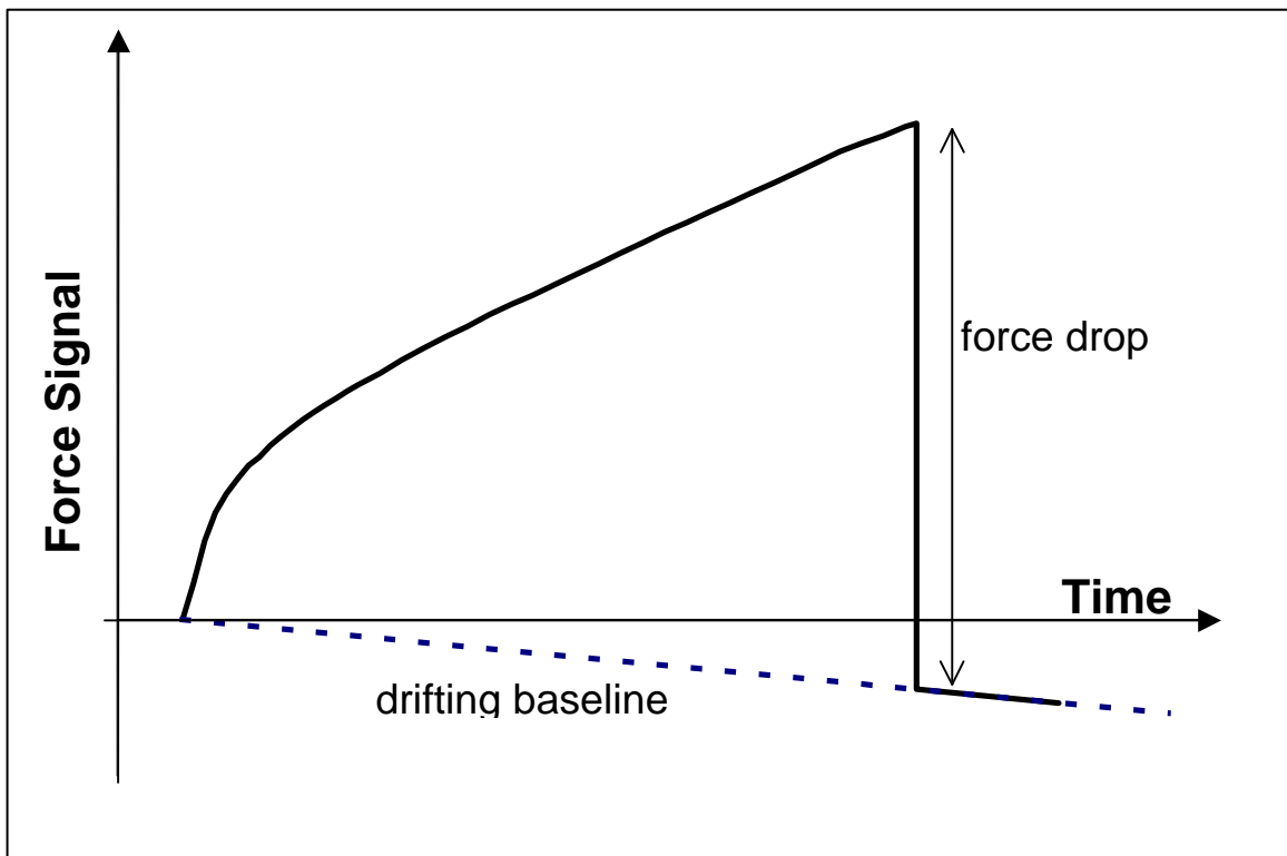
Figure 6: Diagram of Force-Displacement curve showing baseline drift
