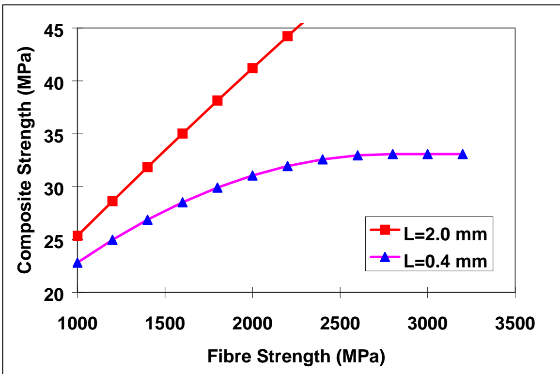
Figure 2: Predicted influence of fibre length and strength on tensile strength of composite
