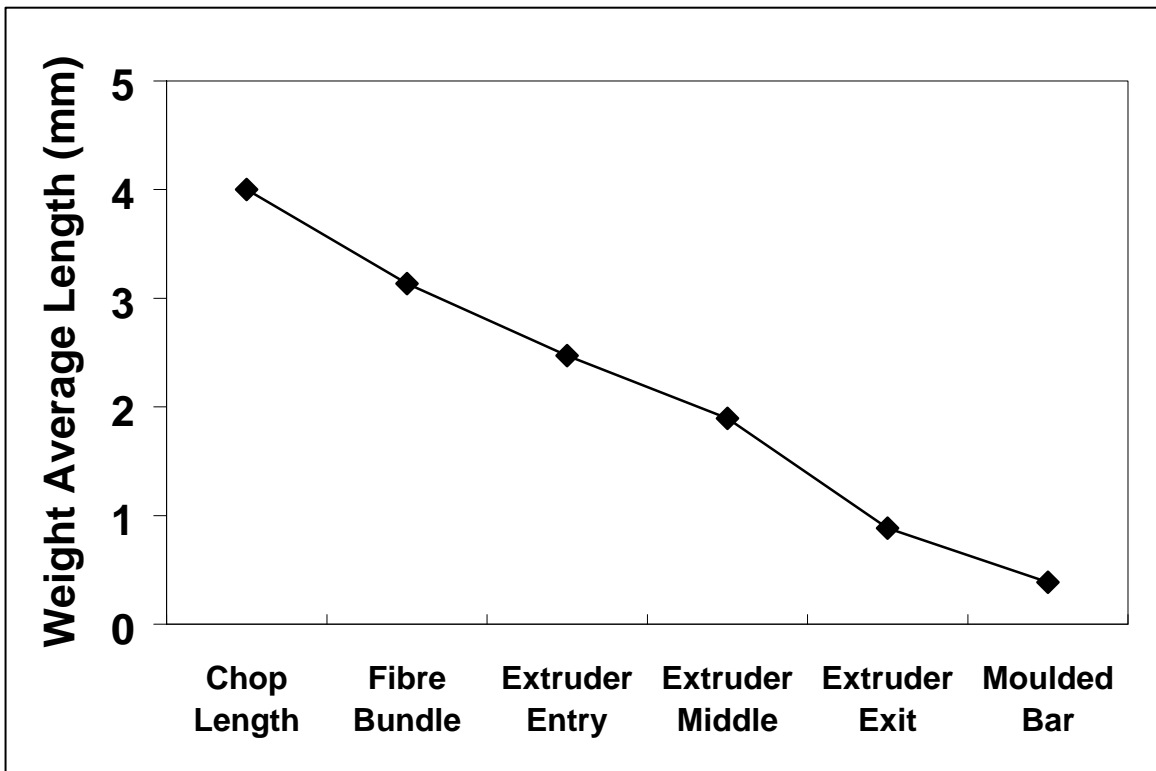
Figure 1: Effect of fibre and composite processing on weight average fibre length
