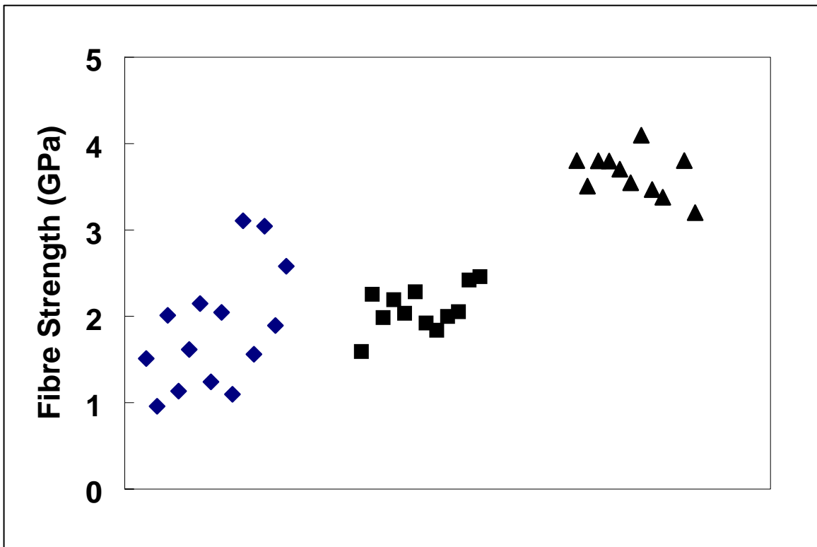
Figure 7: Scatter plot of fibre strength results ( \nu E1, \nu E2, \sigma S)
