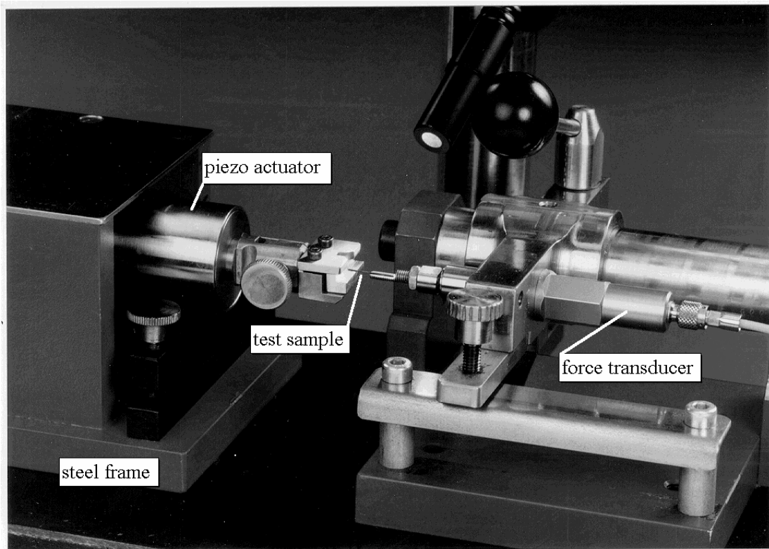
Figure 3: Photograph of the test apparatus
