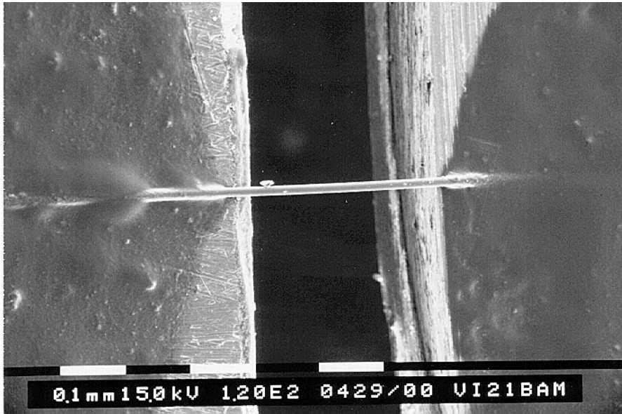
Figure 5: SEM showing glue meniscus on fibre
