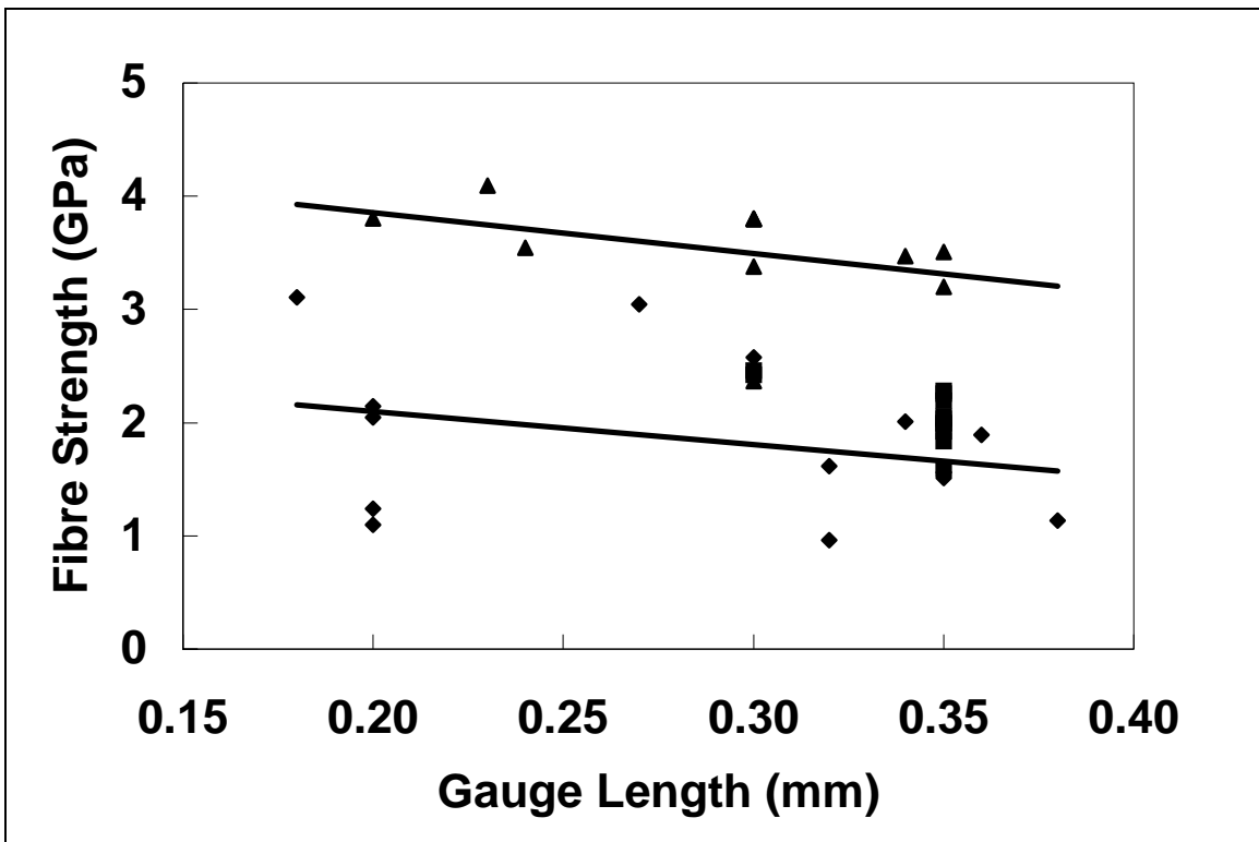
Figure 9: Fibre strength versus gauge length ( \nu E1, \nu E2, \sigma S )
