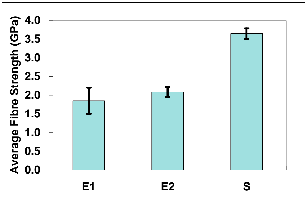
Figure 8: Average fibre strengths and 95% confidence limits
