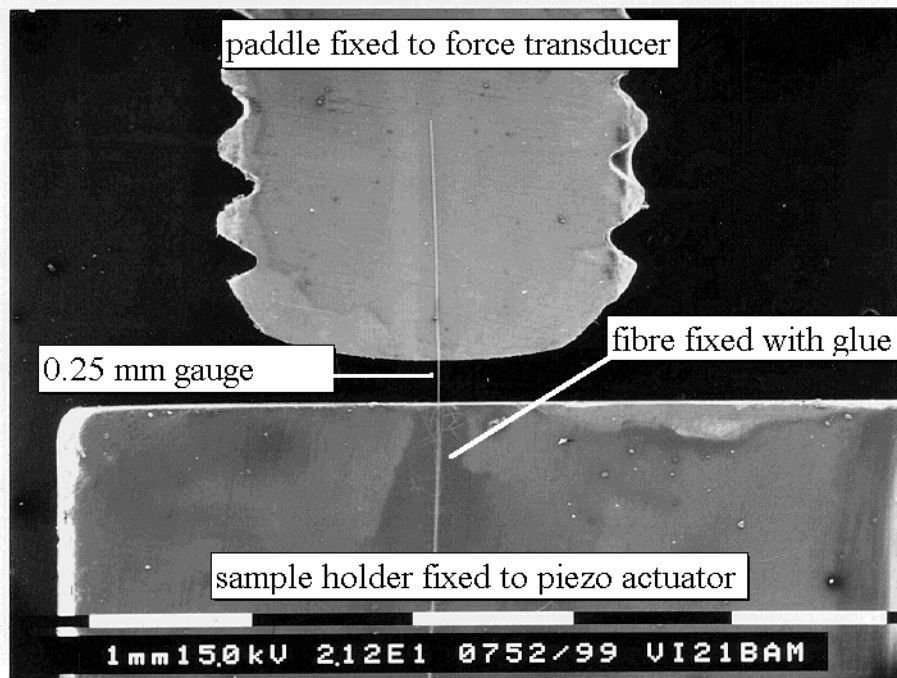
Figure 4: Photograph of basic test arrangement for fibre strength measurement
