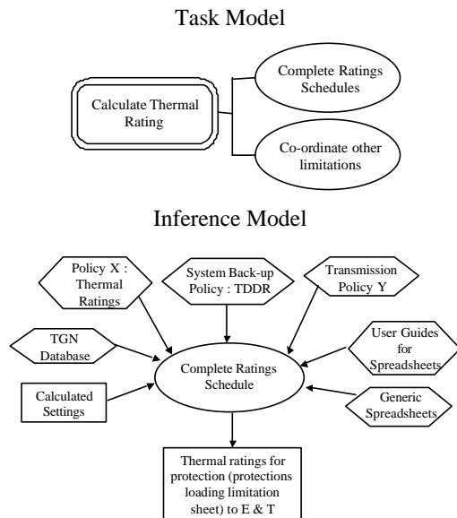
Figure 1: Task and Inference Knowledge Models
