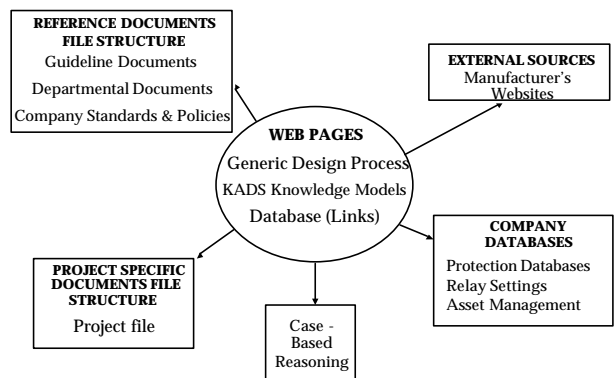
Figure 3: DEKAS Integration with Existing Company Repositories
