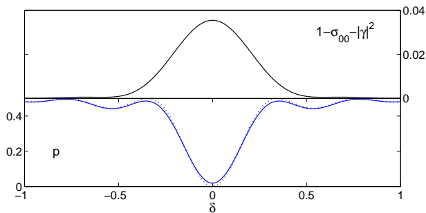
FIG. 1: (Color online) A photon interacting with a dephasing two-level atom via the Jaynes-Cummings model. The solid (dotted) line in the lower panel depicts the probability that a photon is found in the field, as a function of the detuning \delta = \omega - \omega_a , at time t = \pi/(2g) with (without) dephasing. The upper panel shows the excess coherence loss 1 - \sigma_{00} - |\gamma|^2 as a function of detuning \delta in the case with dephasing. Neither the pure Jaynes-Cummings model, nor a simple relaxation model for the atom, gives any excess coherence loss.
