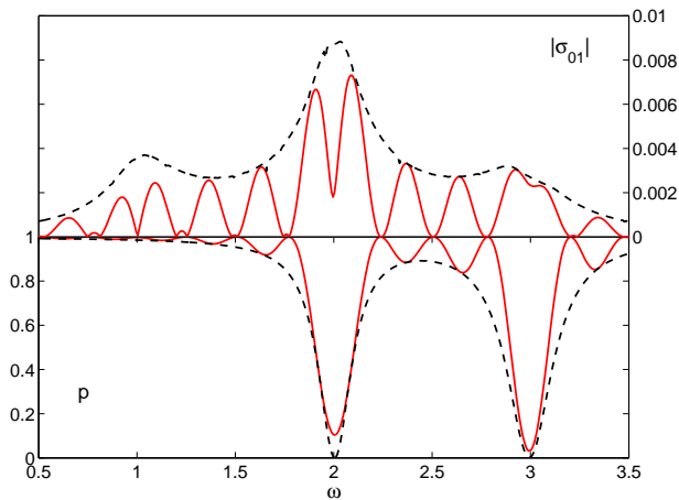
FIG. 2: (Color online) A photon interacting with a three-level atom, according to the Hamiltonian in Eq. (7). The solid line in the lower panel shows the probability p to detect the photon at time t = 25 as a function of the photon energy \omega measured in units of a reference energy \mathcal{E} . The solid line in the upper panel shows the amount of superposition |\sigma_{01}| between the vacuum and a single photon at t = 25 (in units of \mathcal{E}^{-1} ) as a function of \omega . The dashed line in the upper (lower) panel is obtained by at each \omega take the maximum (minimum) of |\sigma_{01}| ( p ) over a long evolution time.
