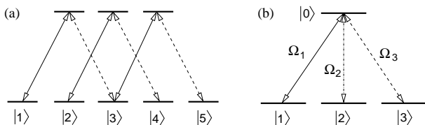
FIG. 1: (a) j = 2 \rightarrow j = 1 transition with two degenerate dark states in the manifolds \{|1\rangle, |3\rangle, |5\rangle\} and \{|2\rangle, |4\rangle\} which are not coupled by non-adiabatic transitions. (b) Tripod coupling scheme forming two degenerate dark states with non-adiabatic coupling.
